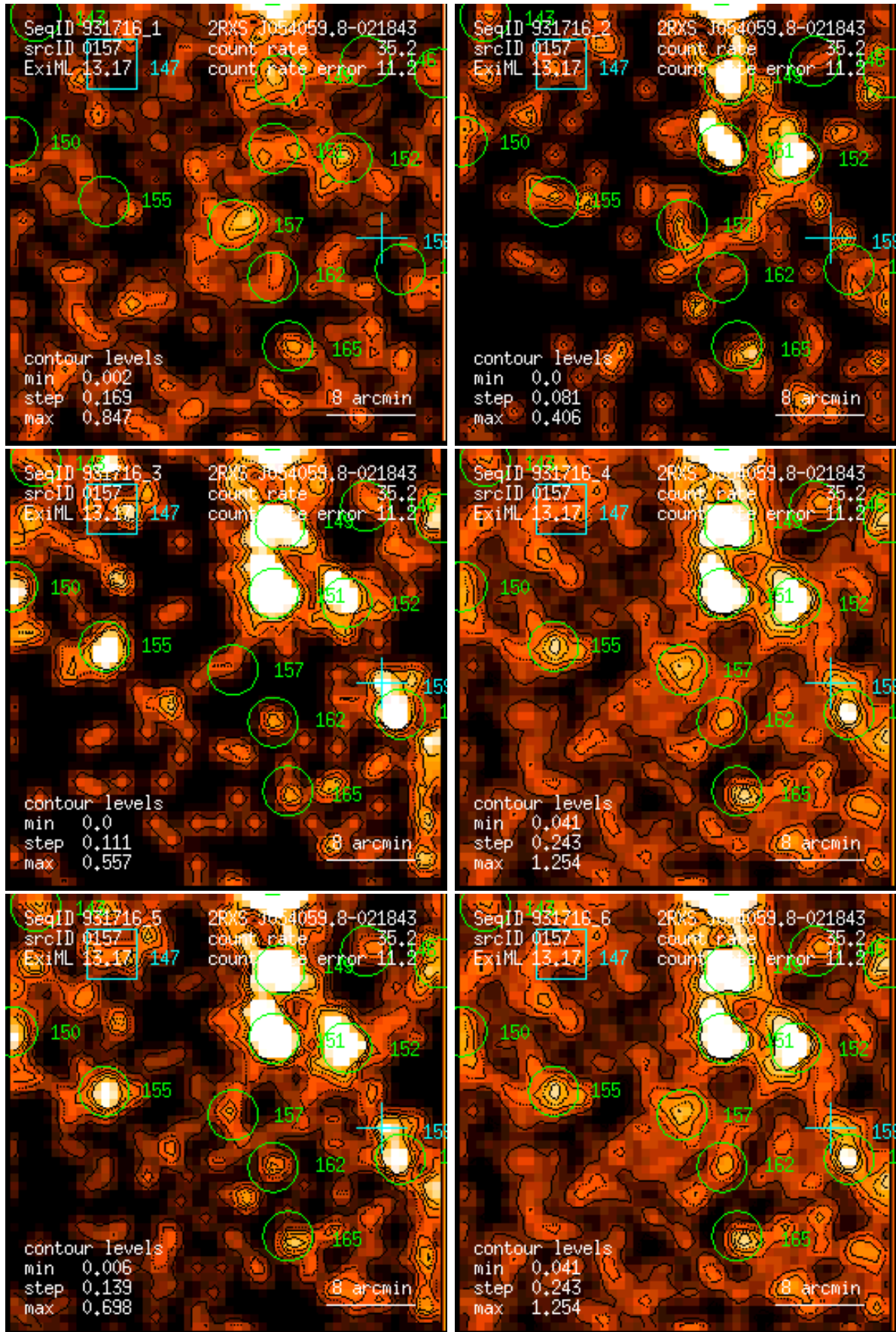
Figure 157: RASS 931716: detection 0157: band rate images, Gaussian filter: (1) PSPC channels 11 – 41, (2) 52 – 90, (3) 91 – 201, (4) 11 – 235, (5) 52 – 201, (6) 11 – 201. Broad band rates in counts/ks. Band rate contour levels in counts/ks/arcmin 2 .
