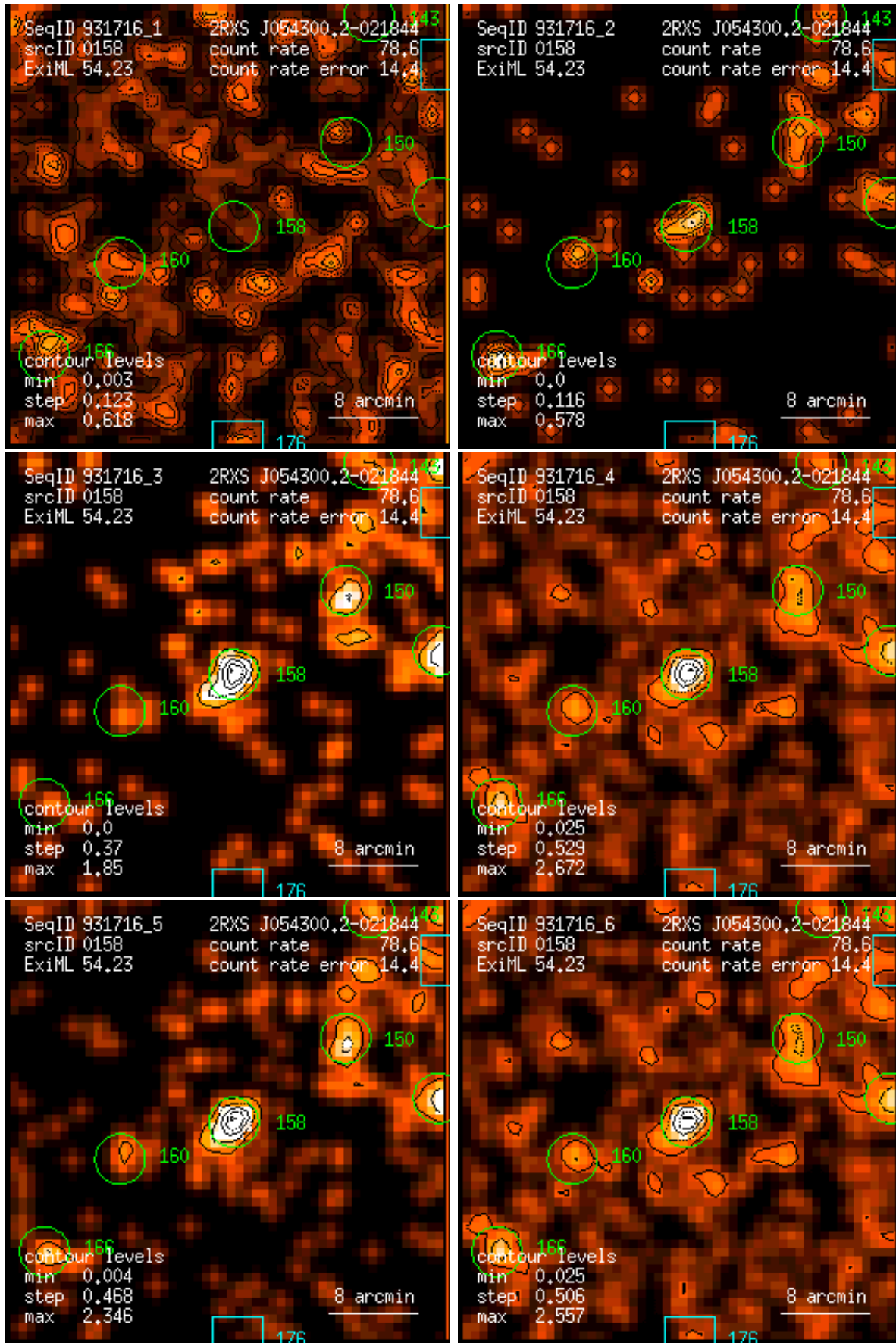
Figure 158: RASS 931716: detection 0158: band rate images, Gaussian filter: (1) PSPC channels 11 – 41, (2) 52 – 90, (3) 91 – 201, (4) 11 – 235, (5) 52 – 201, (6) 11 – 201. Broad band rates in counts/ks. Band rate contour levels in counts/ks/arcmin 2 .
