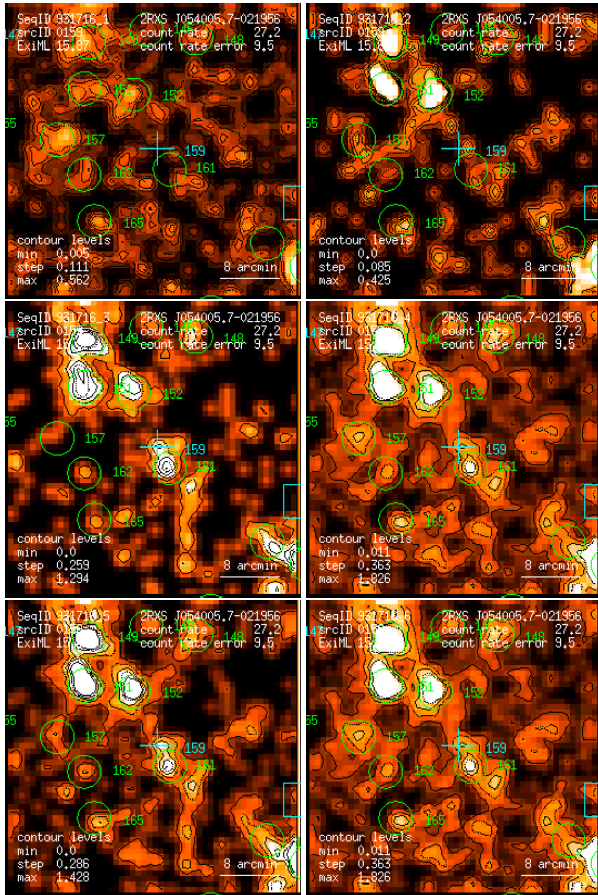
Figure 159: RASS 931716: detection 0159: band rate images, Gaussian filter: (1) PSPC channels 11 – 41, (2) 52 – 90, (3) 91 – 201, (4) 11 – 235, (5) 52 – 201, (6) 11 – 201. Broad band rates in counts/ks. Band rate contour levels in counts/ks/arcmin 2 .
