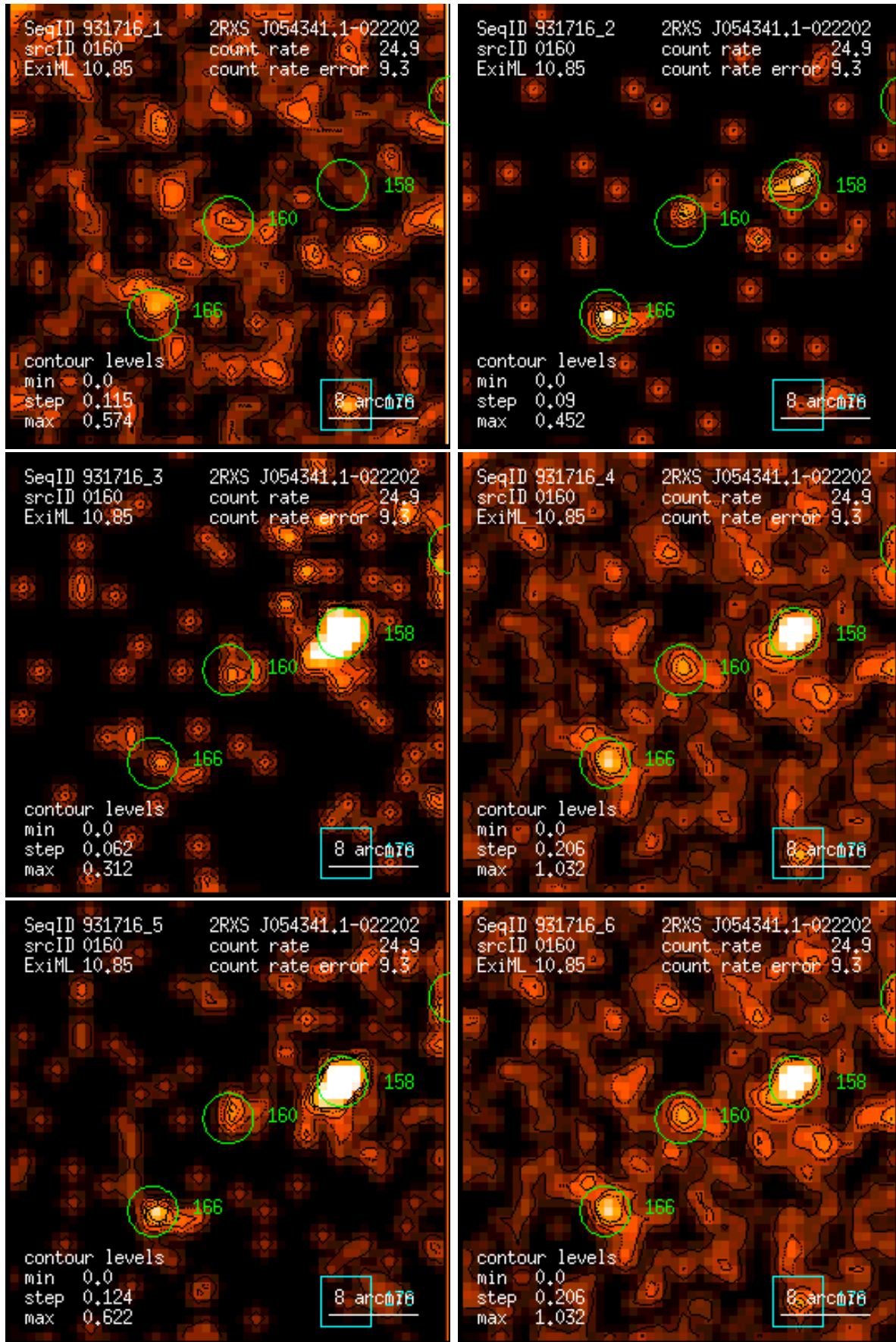
Figure 160: RASS 931716: detection 0160: band rate images, Gaussian filter: (1) PSPC channels 11 – 41, (2) 52 – 90, (3) 91 – 201, (4) 11 – 235, (5) 52 – 201, (6) 11 – 201. Broad band rates in counts/ks. Band rate contour levels in counts/ks/arcmin 2 .
