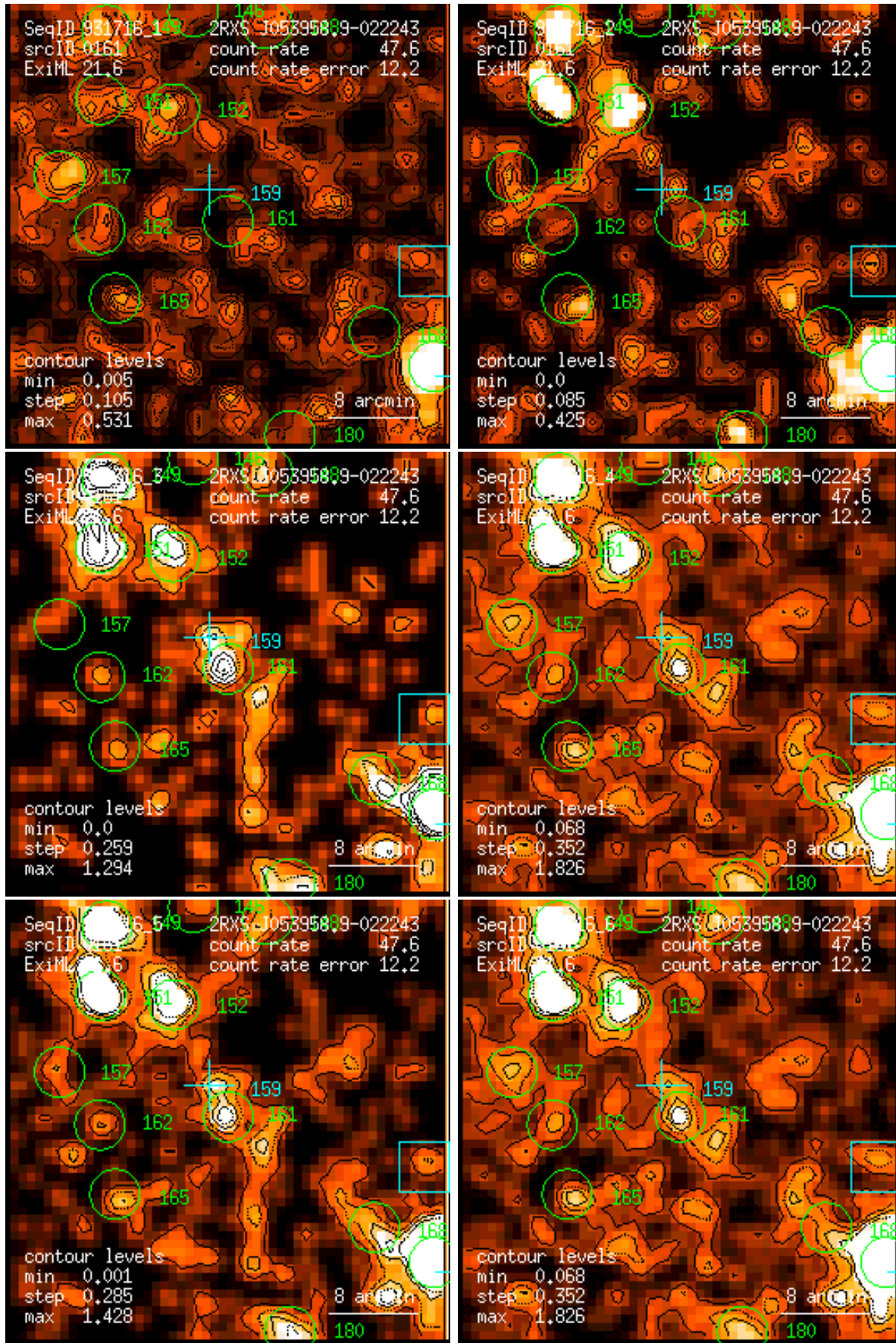
Figure 161: RASS 931716: detection 0161: band rate images, Gaussian filter: (1) PSPC channels 11 – 41, (2) 52 – 90, (3) 91 – 201, (4) 11 – 235, (5) 52 – 201, (6) 11 – 201. Broad band rates in counts/ks. Band rate contour levels in counts/ks/arcmin 2 .
