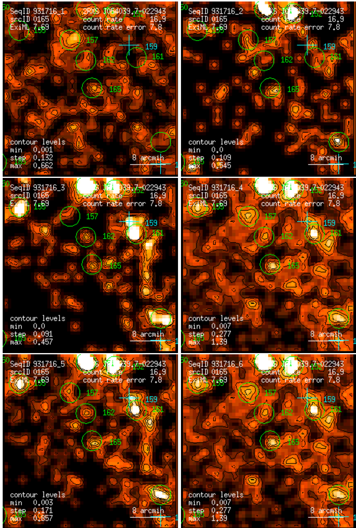
Figure 165: RASS 931716: detection 0165: band rate images, Gaussian filter: (1) PSPC channels 11 – 41, (2) 52 – 90, (3) 91 – 201, (4) 11 – 235, (5) 52 – 201, (6) 11 – 201. Broad band rates in counts/ks. Band rate contour levels in counts/ks/arcmin 2 .
