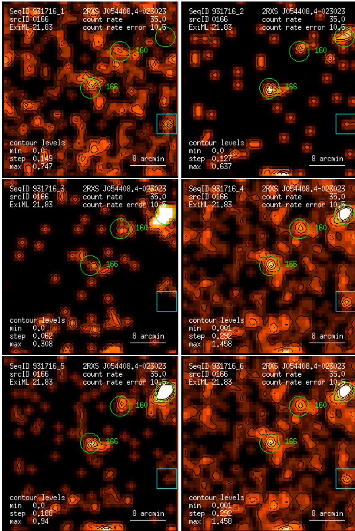
Figure 166: RASS 931716: detection 0166: band rate images, Gaussian filter: (1) PSPC channels 11 – 41, (2) 52 – 90, (3) 91 – 201, (4) 11 – 235, (5) 52 – 201, (6) 11 – 201. Broad band rates in counts/ks. Band rate contour levels in counts/ks/arcmin 2 .
