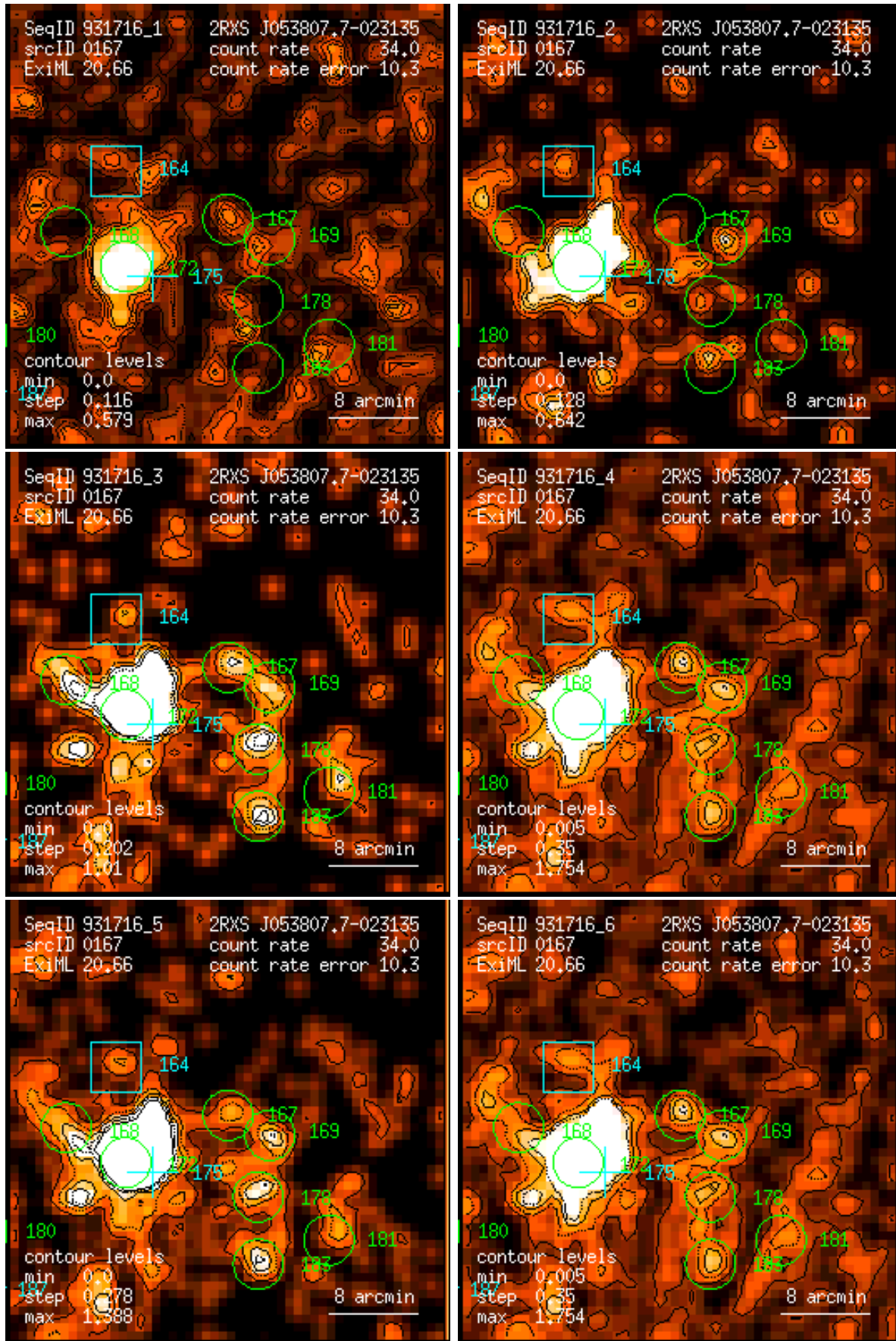
Figure 167: RASS 931716: detection 0167: band rate images, Gaussian filter: (1) PSPC channels 11 – 41, (2) 52 – 90, (3) 91 – 201, (4) 11 – 235, (5) 52 – 201, (6) 11 – 201. Broad band rates in counts/ks. Band rate contour levels in counts/ks/arcmin 2 .
