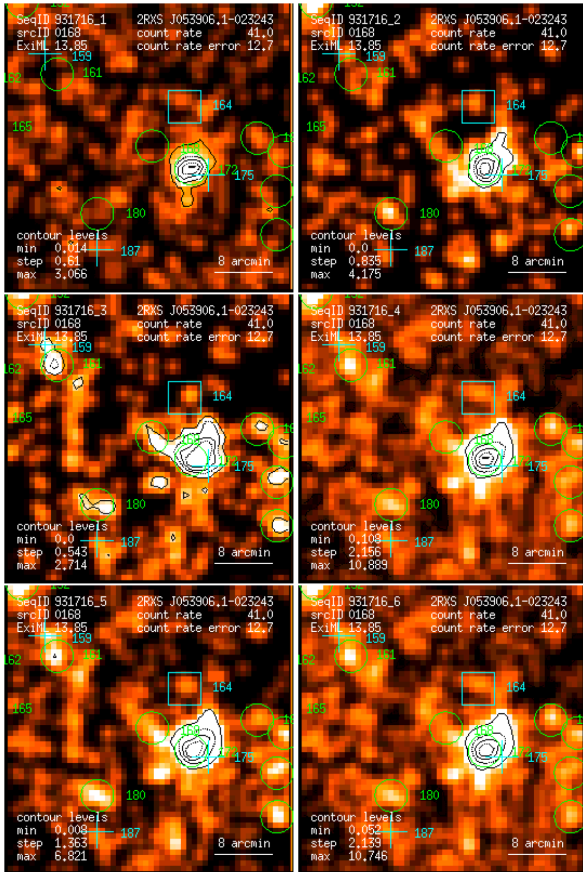
Figure 168: RASS 931716: detection 0168: band rate images, Gaussian filter: (1) PSPC channels 11 – 41, (2) 52 – 90, (3) 91 – 201, (4) 11 – 235, (5) 52 – 201, (6) 11 – 201. Broad band rates in counts/ks. Band rate contour levels in counts/ks/arcmin 2 .
