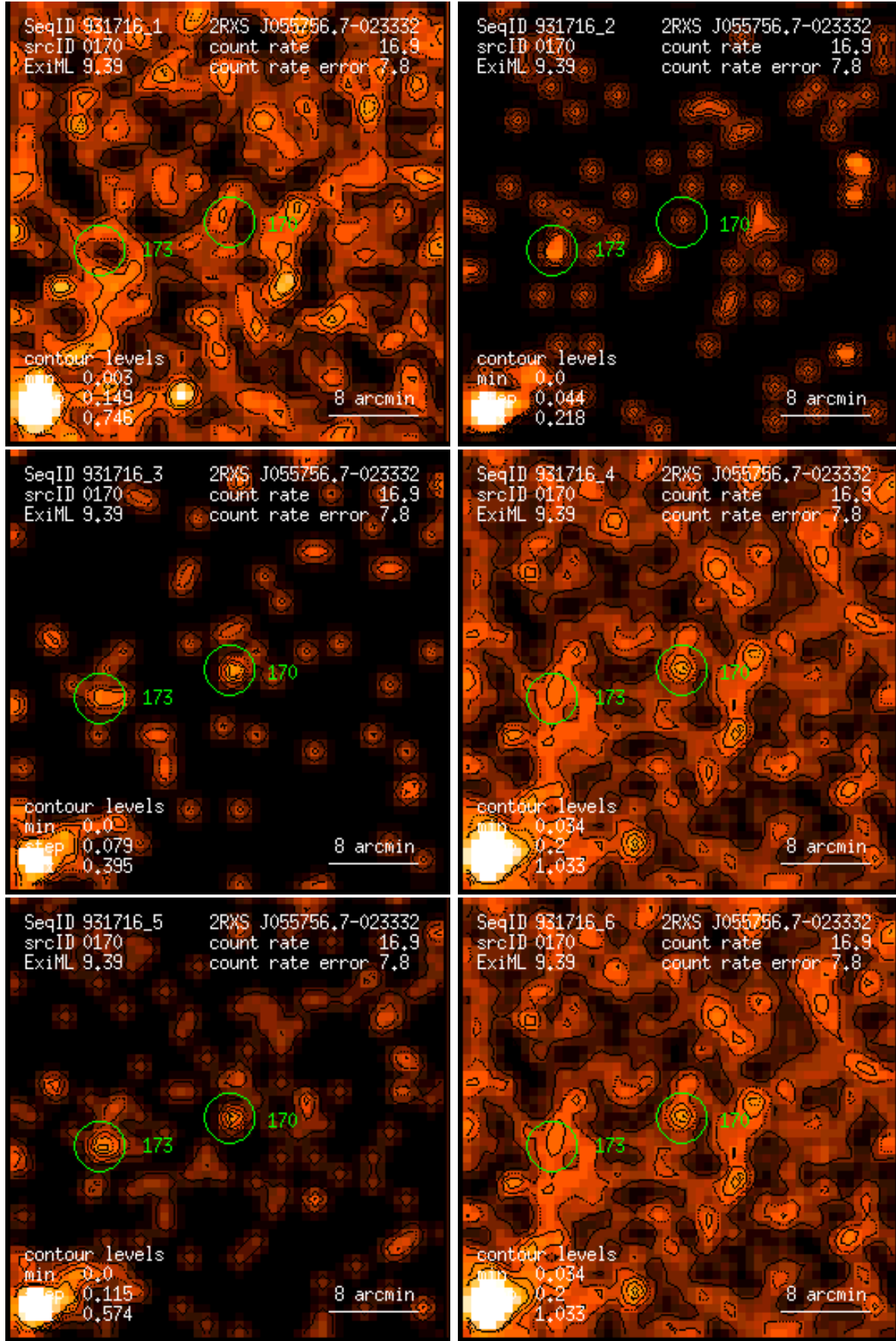
Figure 170: RASS 931716: detection 0170: band rate images, Gaussian filter: (1) PSPC channels 11 – 41, (2) 52 – 90, (3) 91 – 201, (4) 11 – 235, (5) 52 – 201, (6) 11 – 201. Broad band rates in counts/ks. Band rate contour levels in counts/ks/arcmin 2 .
