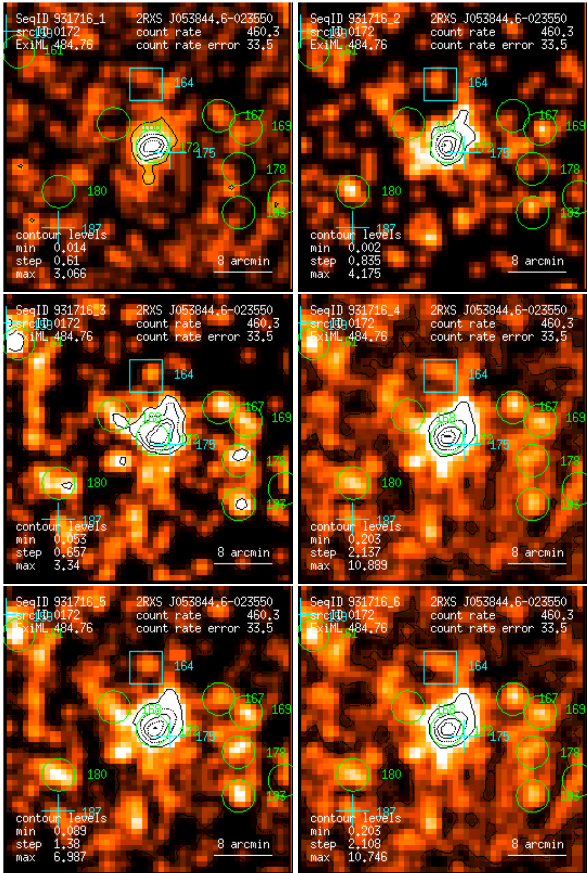
Figure 172: RASS 931716: detection 0172: band rate images, Gaussian filter: (1) PSPC channels 11 – 41, (2) 52 – 90, (3) 91 – 201, (4) 11 – 235, (5) 52 – 201, (6) 11 – 201. Broad band rates in counts/ks. Band rate contour levels in counts/ks/arcmin 2 .
