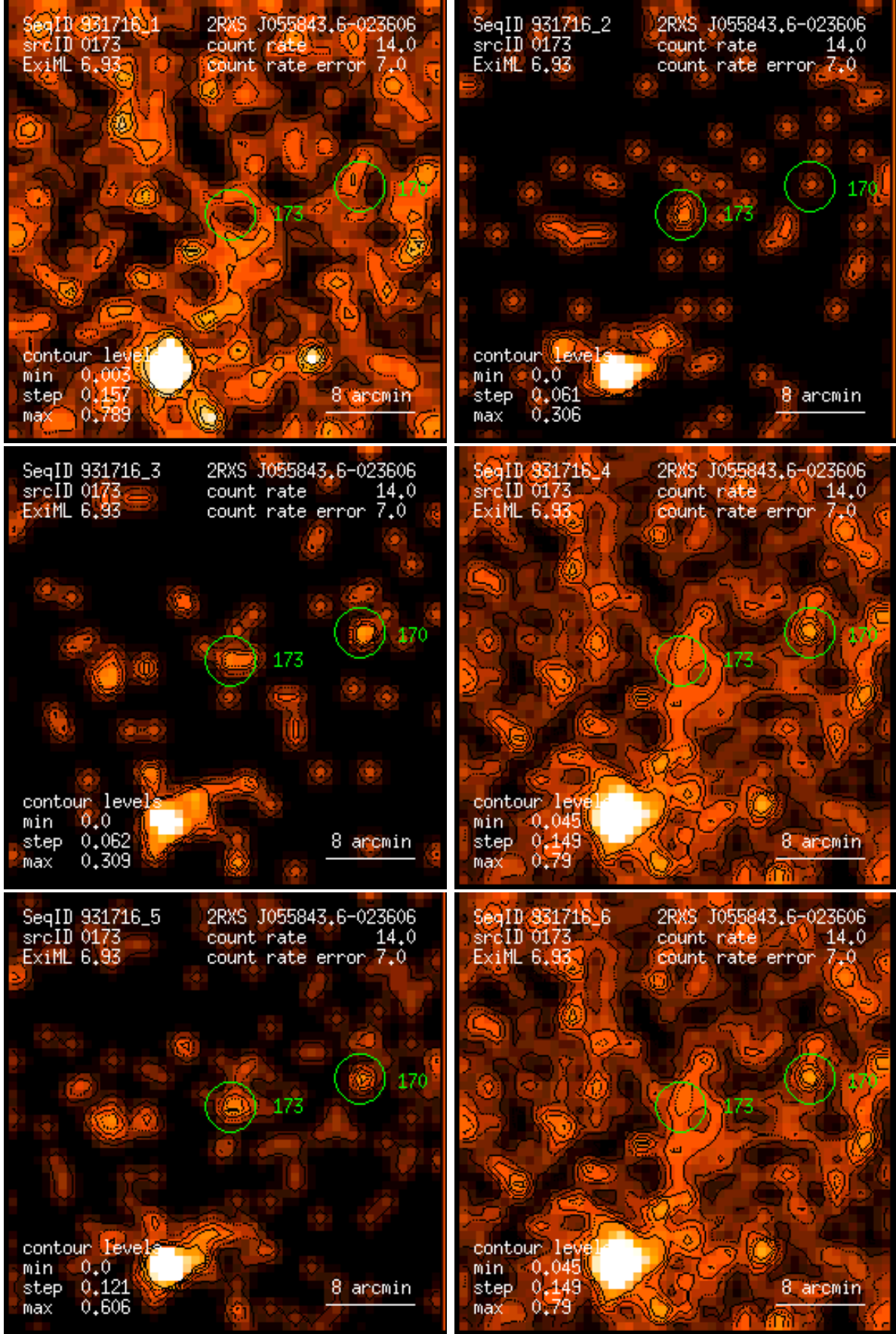
Figure 173: RASS 931716: detection 0173: band rate images, Gaussian filter: (1) PSPC channels 11 – 41, (2) 52 – 90, (3) 91 – 201, (4) 11 – 235, (5) 52 – 201, (6) 11 – 201. Broad band rates in counts/ks. Band rate contour levels in counts/ks/arcmin 2 .
