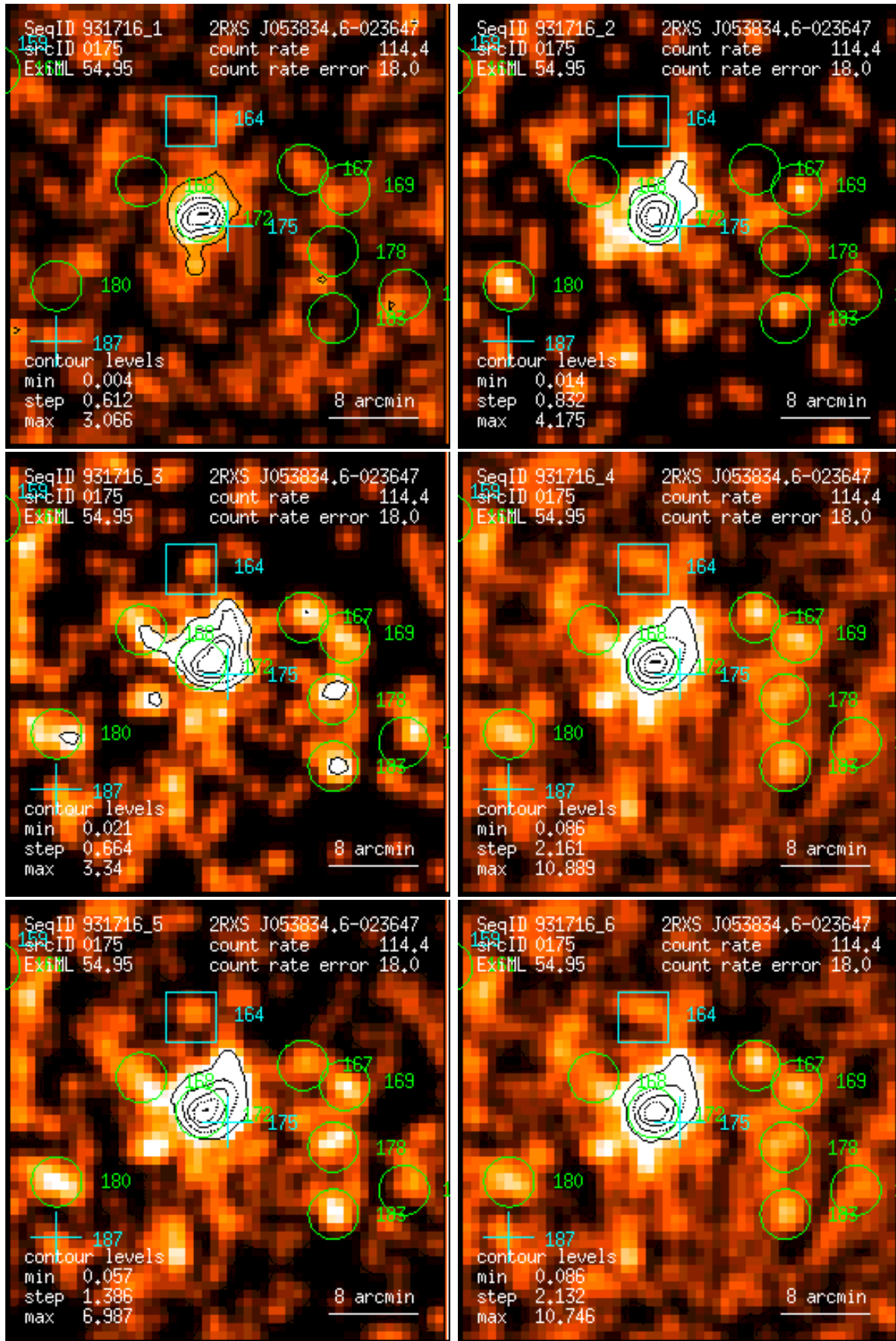
Figure 175: RASS 931716: detection 0175: band rate images, Gaussian filter: (1) PSPC channels 11 – 41, (2) 52 – 90, (3) 91 – 201, (4) 11 – 235, (5) 52 – 201, (6) 11 – 201. Broad band rates in counts/ks. Band rate contour levels in counts/ks/arcmin 2 .
