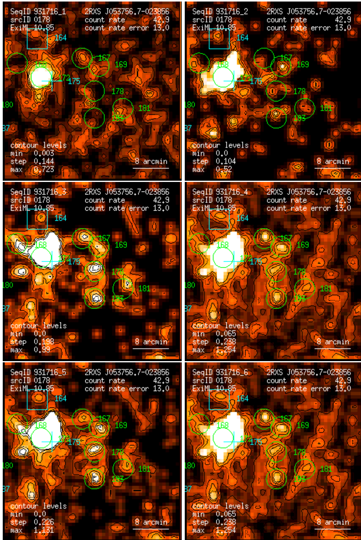
Figure 178: RASS 931716: detection 0178: band rate images, Gaussian filter: (1) PSPC channels 11 – 41, (2) 52 – 90, (3) 91 – 201, (4) 11 – 235, (5) 52 – 201, (6) 11 – 201. Broad band rates in counts/ks. Band rate contour levels in counts/ks/arcmin 2 .
