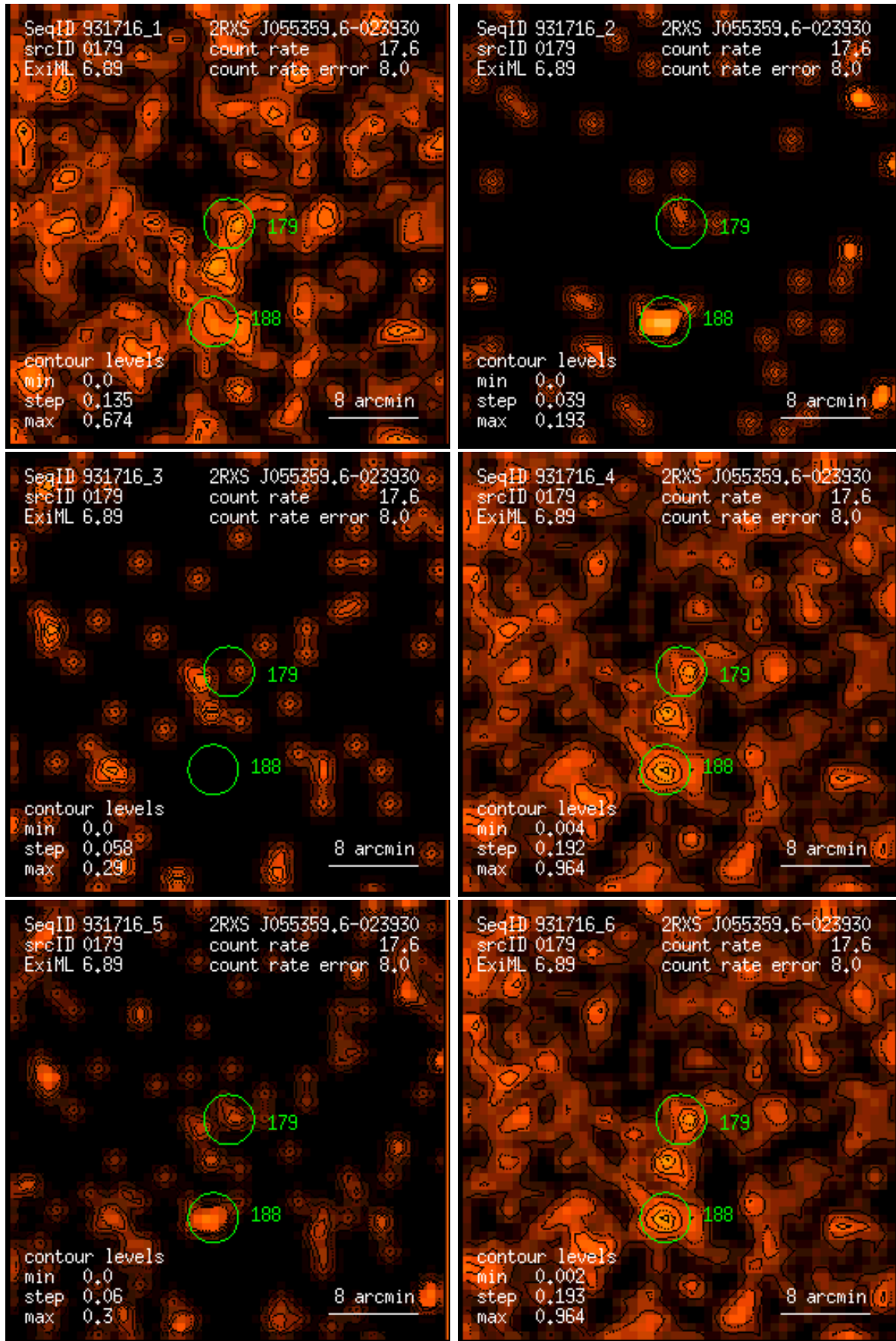
Figure 179: RASS 931716: detection 0179: band rate images, Gaussian filter: (1) PSPC channels 11 – 41, (2) 52 – 90, (3) 91 – 201, (4) 11 – 235, (5) 52 – 201, (6) 11 – 201. Broad band rates in counts/ks. Band rate contour levels in counts/ks/arcmin 2 .
