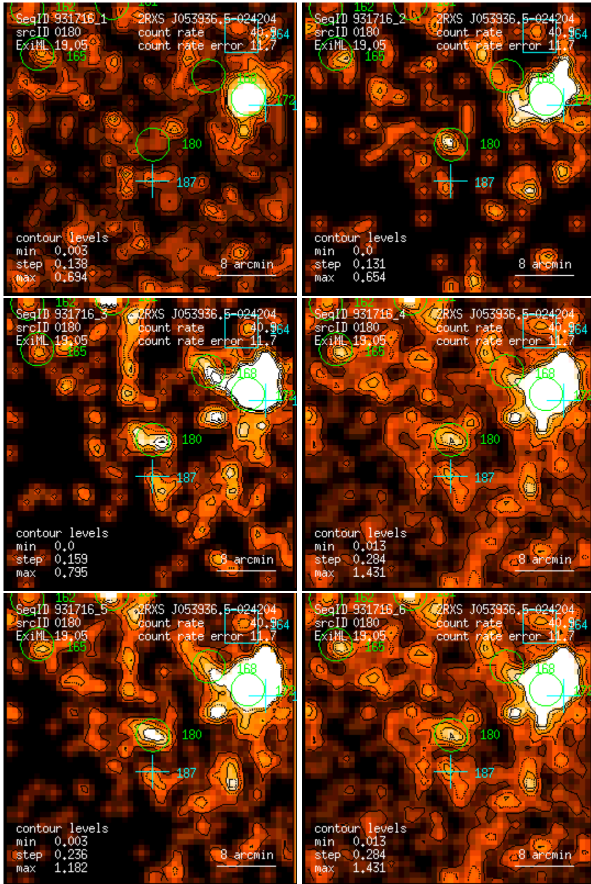
Figure 180: RASS 931716: detection 0180: band rate images, Gaussian filter: (1) PSPC channels 11 – 41, (2) 52 – 90, (3) 91 – 201, (4) 11 – 235, (5) 52 – 201, (6) 11 – 201. Broad band rates in counts/ks. Band rate contour levels in counts/ks/arcmin 2 .
