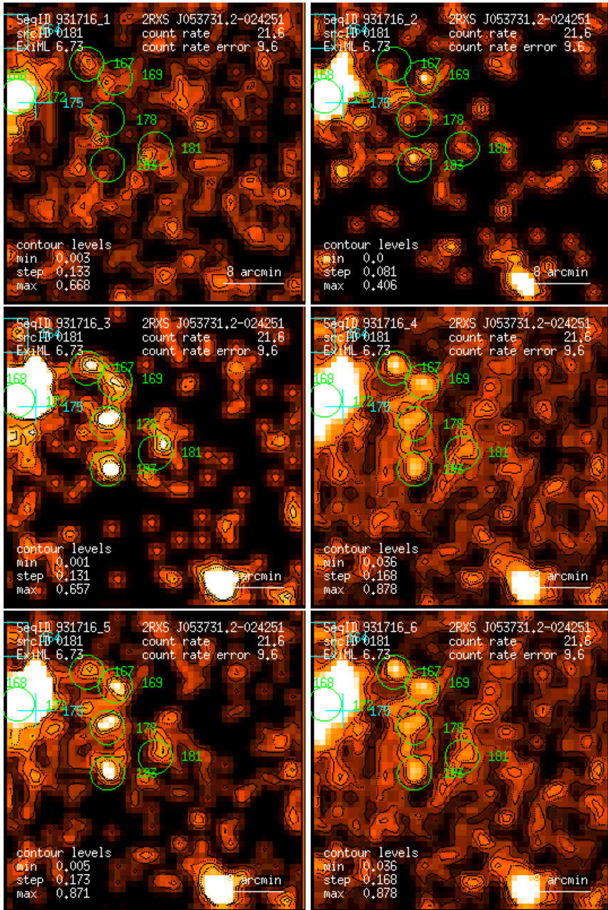
Figure 181: RASS 931716: detection 0181: band rate images, Gaussian filter: (1) PSPC channels 11 – 41, (2) 52 – 90, (3) 91 – 201, (4) 11 – 235, (5) 52 – 201, (6) 11 – 201. Broad band rates in counts/ks. Band rate contour levels in counts/ks/arcmin 2 .
