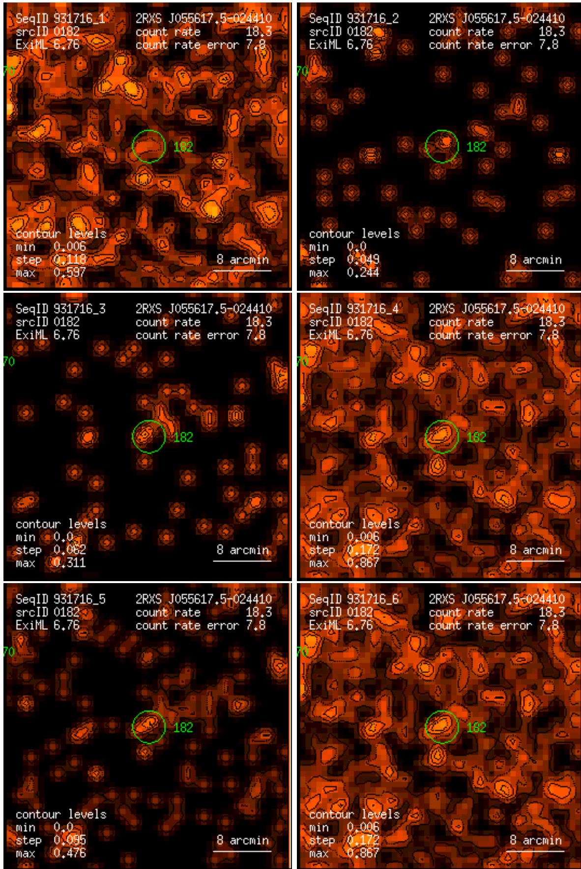
Figure 182: RASS 931716: detection 0182: band rate images, Gaussian filter: (1) PSPC channels 11 – 41, (2) 52 – 90, (3) 91 – 201, (4) 11 – 235, (5) 52 – 201, (6) 11 – 201. Broad band rates in counts/ks. Band rate contour levels in counts/ks/arcmin 2 .
