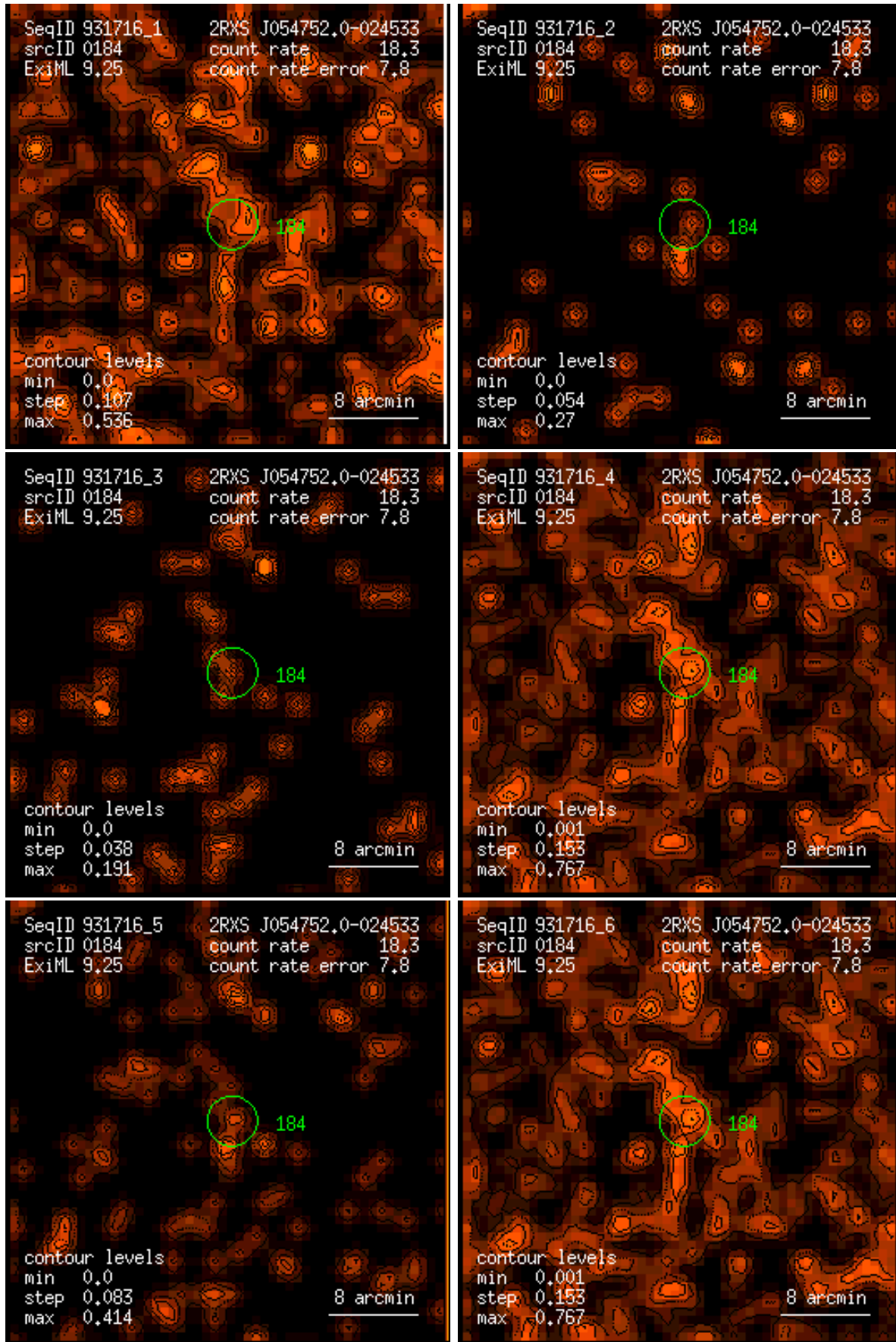
Figure 184: RASS 931716: detection 0184: band rate images, Gaussian filter: (1) PSPC channels 11 – 41, (2) 52 – 90, (3) 91 – 201, (4) 11 – 235, (5) 52 – 201, (6) 11 – 201. Broad band rates in counts/ks. Band rate contour levels in counts/ks/arcmin 2 .
