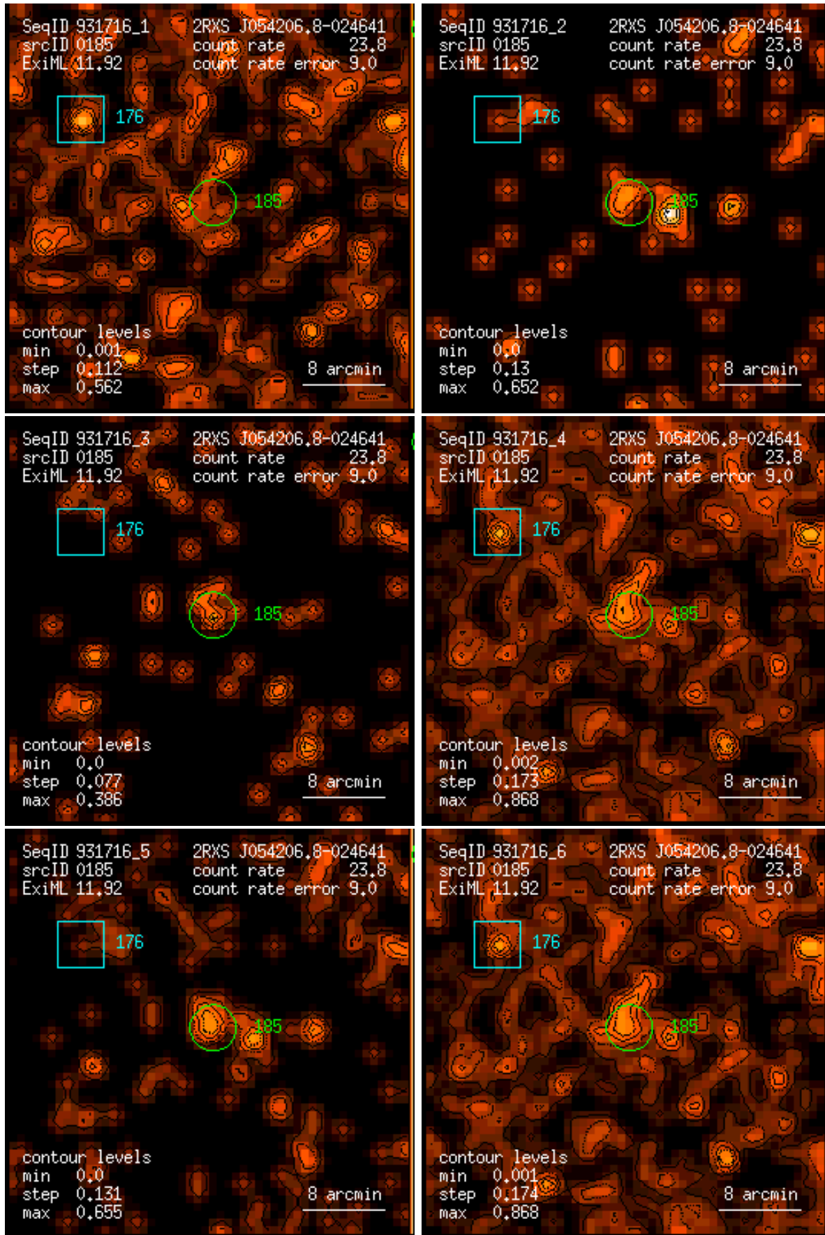
Figure 185: RASS 931716: detection 0185: band rate images, Gaussian filter: (1) PSPC channels 11 – 41, (2) 52 – 90, (3) 91 – 201, (4) 11 – 235, (5) 52 – 201, (6) 11 – 201. Broad band rates in counts/ks. Band rate contour levels in counts/ks/arcmin 2 .
