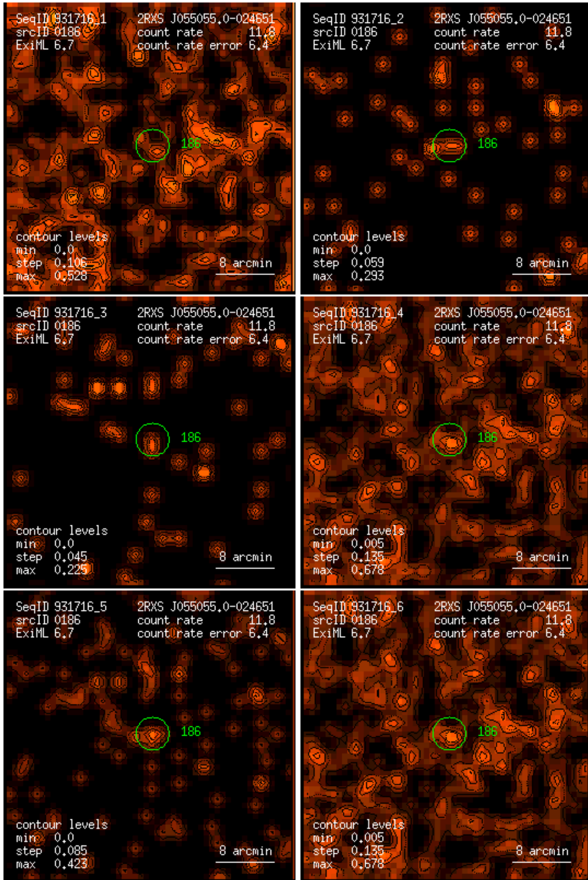
Figure 186: RASS 931716: detection 0186: band rate images, Gaussian filter: (1) PSPC channels 11 – 41, (2) 52 – 90, (3) 91 – 201, (4) 11 – 235, (5) 52 – 201, (6) 11 – 201. Broad band rates in counts/ks. Band rate contour levels in counts/ks/arcmin 2 .
