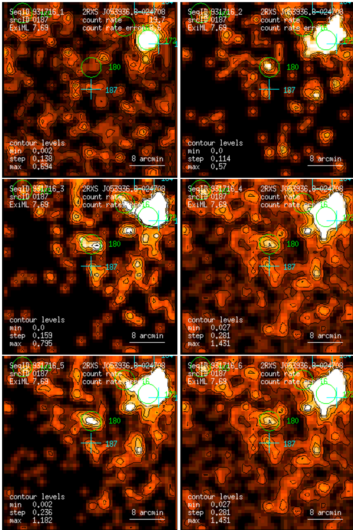
Figure 187: RASS 931716: detection 0187: band rate images, Gaussian filter: (1) PSPC channels 11 – 41, (2) 52 – 90, (3) 91 – 201, (4) 11 – 235, (5) 52 – 201, (6) 11 – 201. Broad band rates in counts/ks. Band rate contour levels in counts/ks/arcmin 2 .
