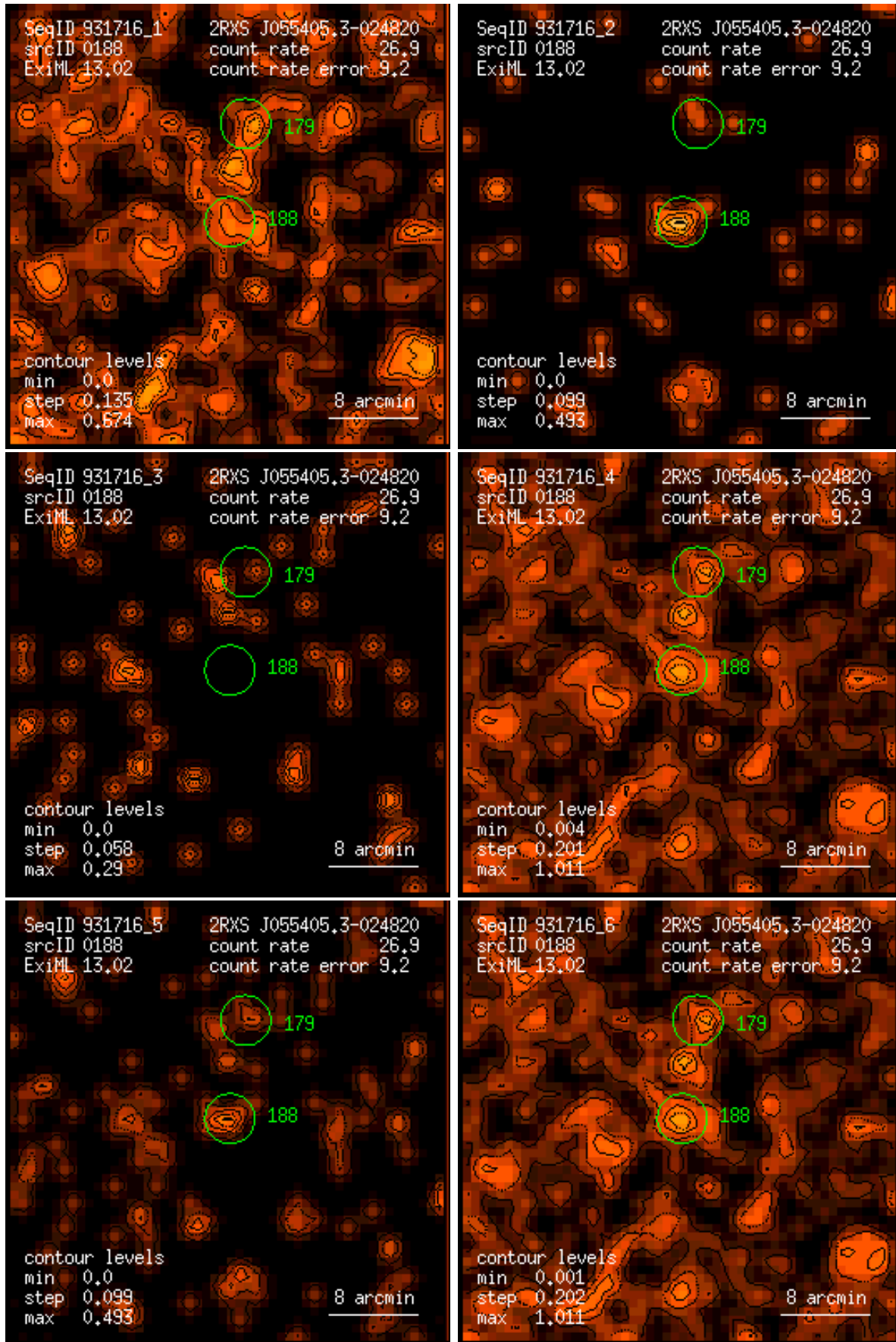
Figure 188: RASS 931716: detection 0188: band rate images, Gaussian filter: (1) PSPC channels 11 – 41, (2) 52 – 90, (3) 91 – 201, (4) 11 – 235, (5) 52 – 201, (6) 11 – 201. Broad band rates in counts/ks. Band rate contour levels in counts/ks/arcmin 2 .
