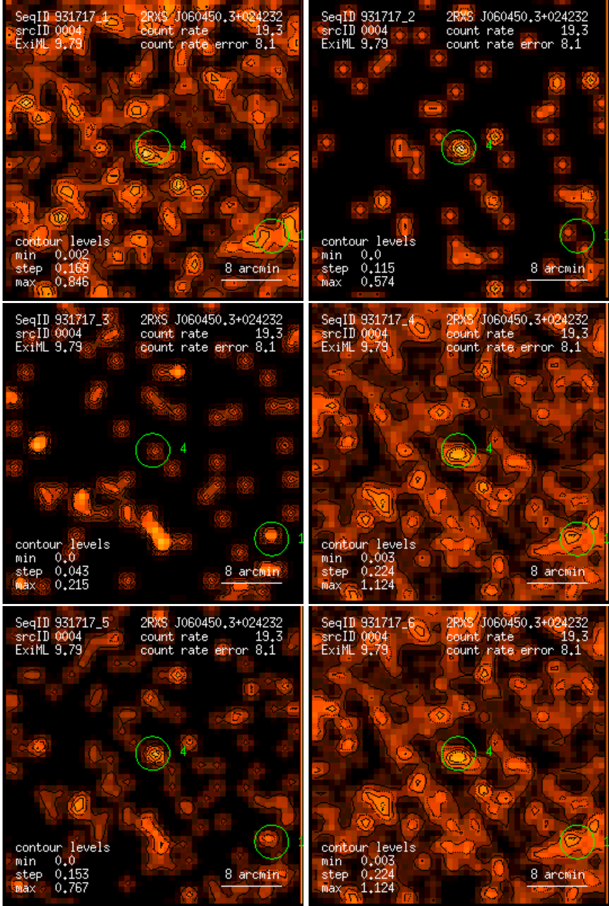
Figure 4: RASS 931717: detection 0004: band rate images, Gaussian filter: (1) PSPC channels 11 – 41, (2) 52 – 90, (3) 91 – 201, (4) 11 – 235, (5) 52 – 201, (6) 11 – 201. Broad band rates in counts/ks. Band rate contour levels in counts/ks/arcmin 2 .
