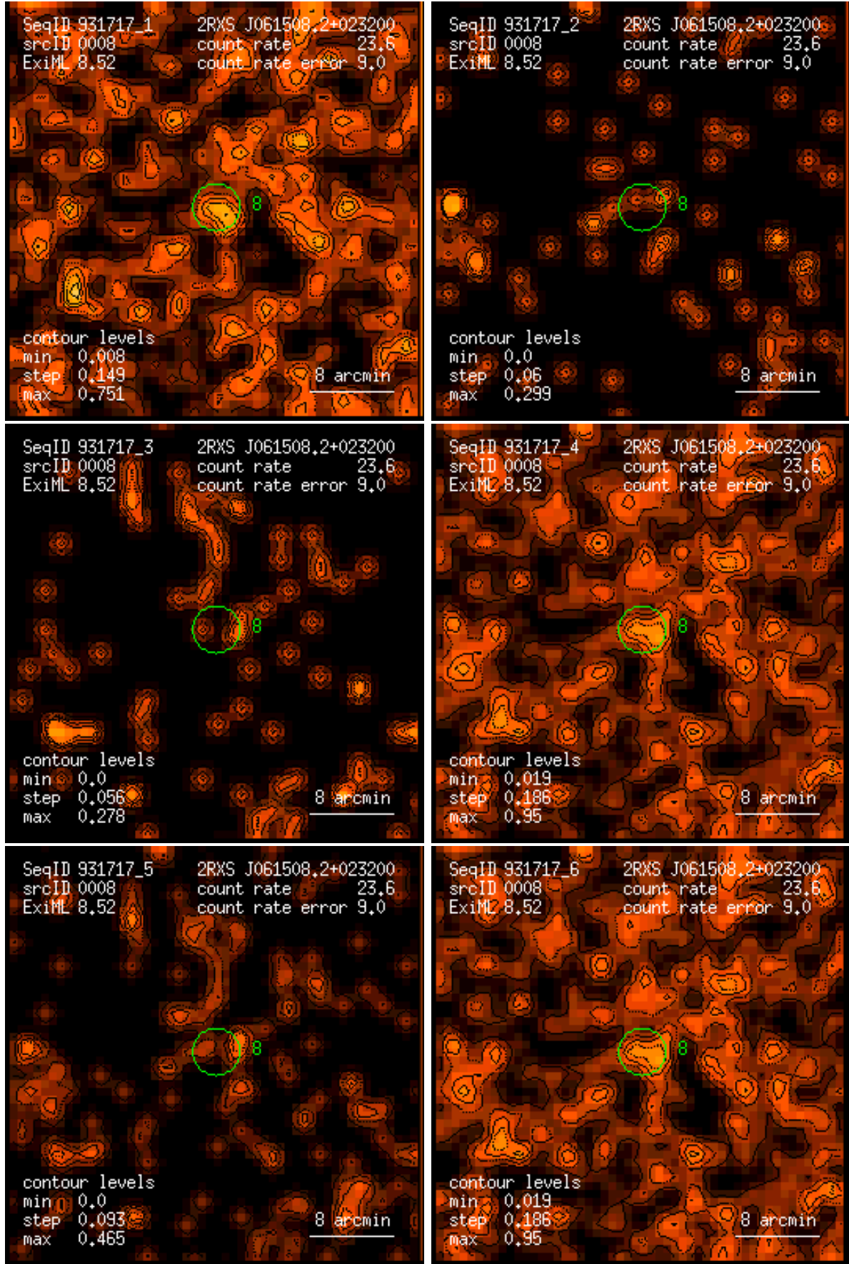
Figure 8: RASS 931717: detection 0008: band rate images, Gaussian filter: (1) PSPC channels 11 – 41, (2) 52 – 90, (3) 91 – 201, (4) 11 – 235, (5) 52 – 201, (6) 11 – 201. Broad band rates in counts/ks. Band rate contour levels in counts/ks/arcmin 2 .
