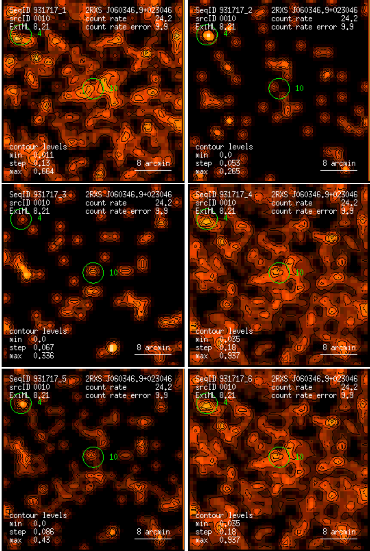
Figure 10: RASS 931717: detection 0010: band rate images, Gaussian filter: (1) PSPC channels 11 – 41, (2) 52 – 90, (3) 91 – 201, (4) 11 – 235, (5) 52 – 201, (6) 11 – 201. Broad band rates in counts/ks. Band rate contour levels in counts/ks/arcmin 2 .
