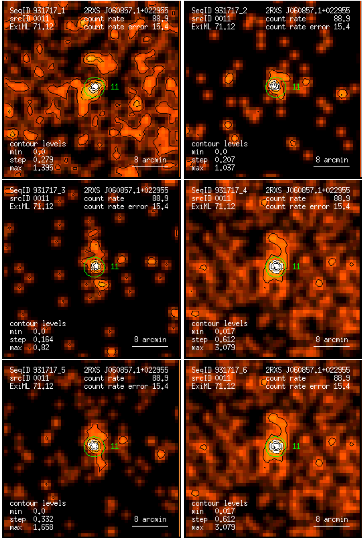
Figure 11: RASS 931717: detection 0011: band rate images, Gaussian filter: (1) PSPC channels 11 – 41, (2) 52 – 90, (3) 91 – 201, (4) 11 – 235, (5) 52 – 201, (6) 11 – 201. Broad band rates in counts/ks. Band rate contour levels in counts/ks/arcmin 2 .
