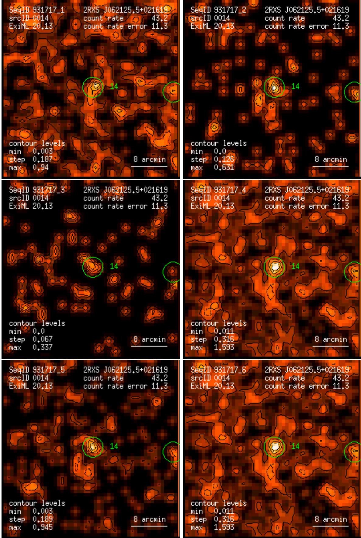
Figure 14: RASS 931717: detection 0014: band rate images, Gaussian filter: (1) PSPC channels 11 – 41, (2) 52 – 90, (3) 91 – 201, (4) 11 – 235, (5) 52 – 201, (6) 11 – 201. Broad band rates in counts/ks. Band rate contour levels in counts/ks/arcmin 2 .
