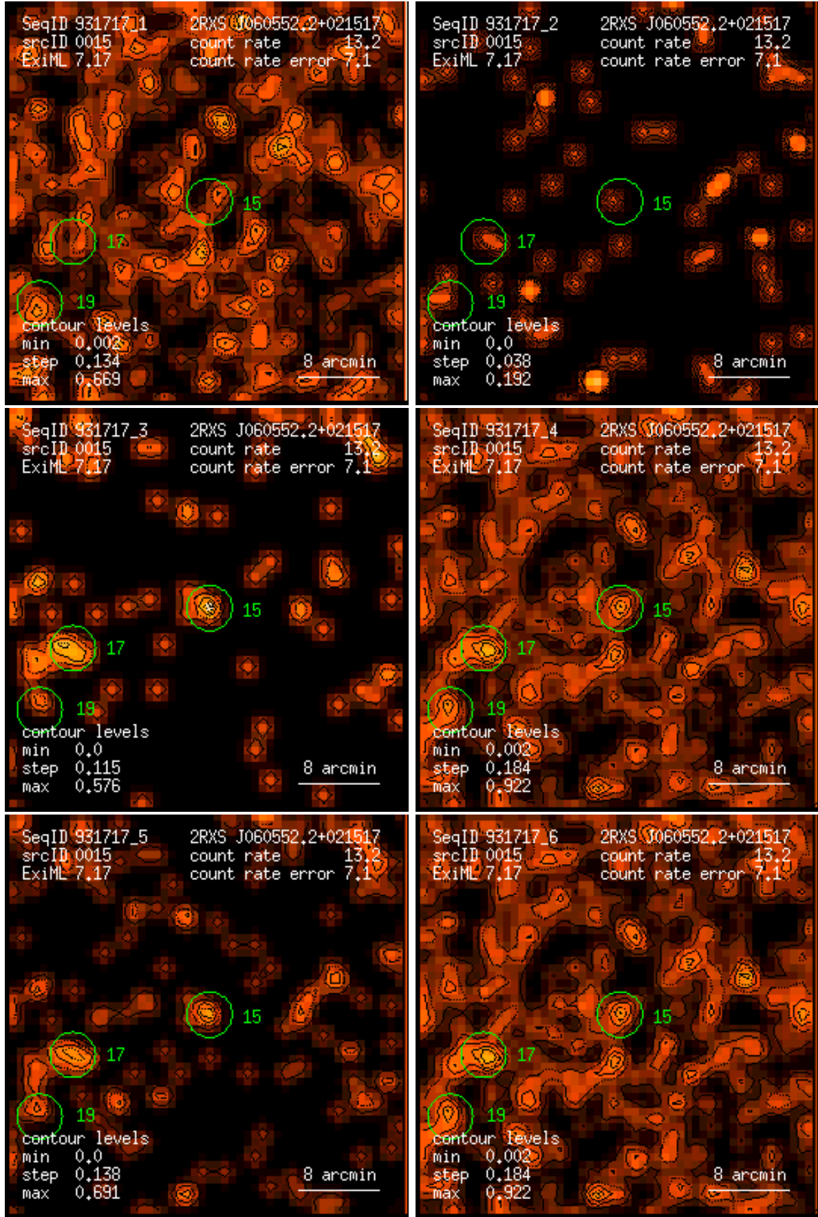
Figure 15: RASS 931717: detection 0015: band rate images, Gaussian filter: (1) PSPC channels 11 – 41, (2) 52 – 90, (3) 91 – 201, (4) 11 – 235, (5) 52 – 201, (6) 11 – 201. Broad band rates in counts/ks. Band rate contour levels in counts/ks/arcmin 2 .
