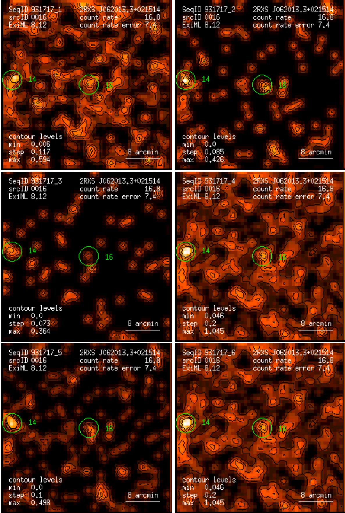
Figure 16: RASS 931717: detection 0016: band rate images, Gaussian filter: (1) PSPC channels 11 – 41, (2) 52 – 90, (3) 91 – 201, (4) 11 – 235, (5) 52 – 201, (6) 11 – 201. Broad band rates in counts/ks. Band rate contour levels in counts/ks/arcmin 2 .
