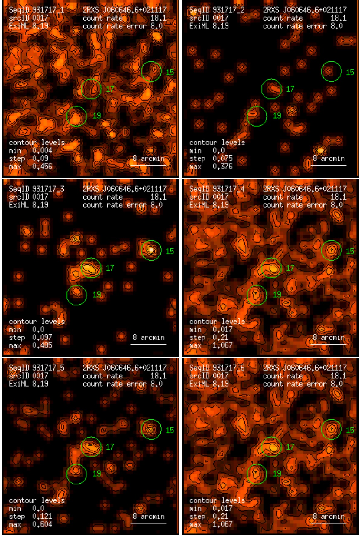
Figure 17: RASS 931717: detection 0017: band rate images, Gaussian filter: (1) PSPC channels 11 – 41, (2) 52 – 90, (3) 91 – 201, (4) 11 – 235, (5) 52 – 201, (6) 11 – 201. Broad band rates in counts/ks. Band rate contour levels in counts/ks/arcmin 2 .
