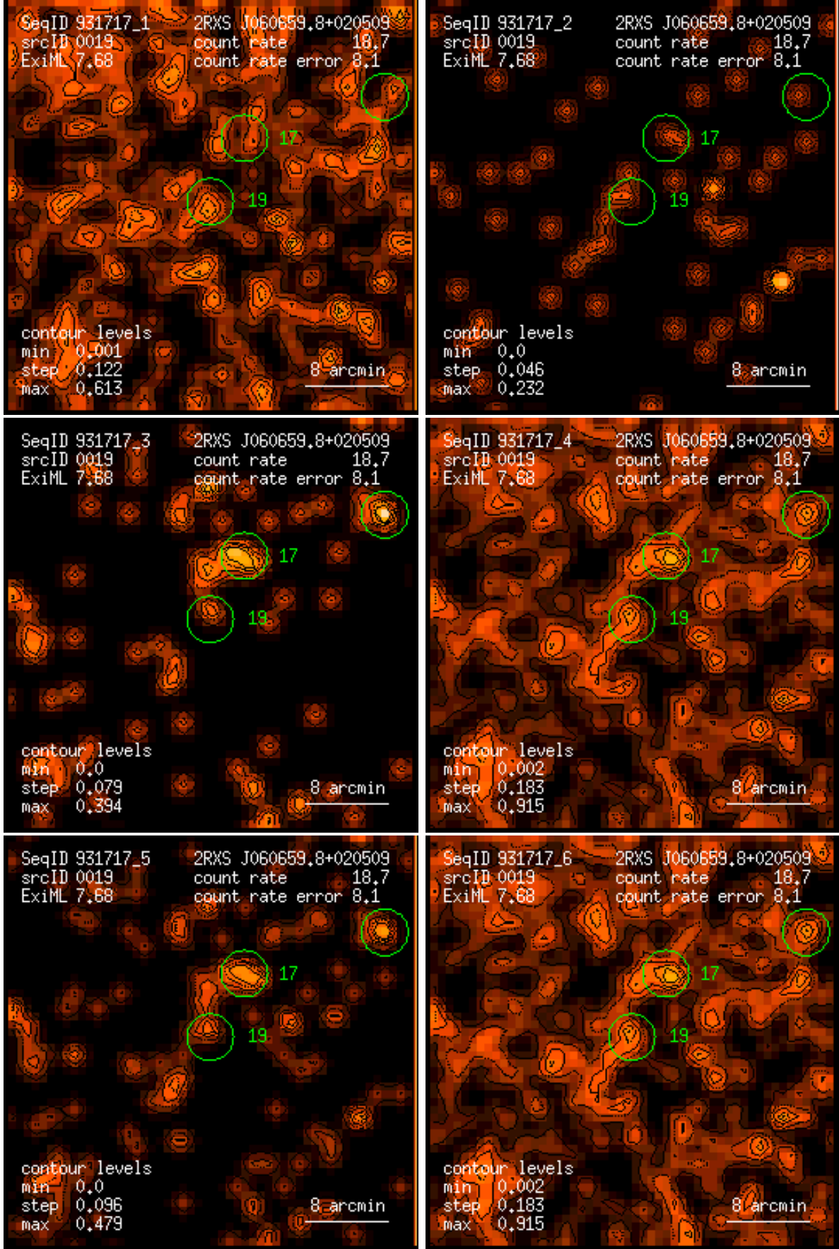
Figure 19: RASS 931717: detection 0019: band rate images, Gaussian filter: (1) PSPC channels 11 – 41, (2) 52 – 90, (3) 91 – 201, (4) 11 – 235, (5) 52 – 201, (6) 11 – 201. Broad band rates in counts/ks. Band rate contour levels in counts/ks/arcmin 2 .
