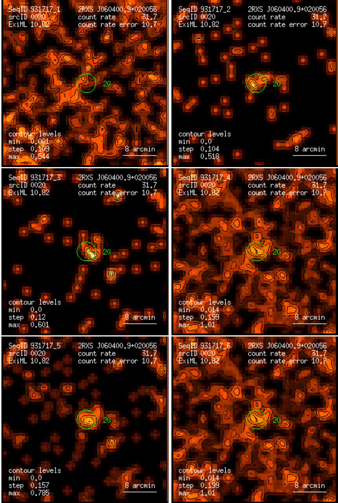
Figure 20: RASS 931717: detection 0020: band rate images, Gaussian filter: (1) PSPC channels 11 – 41, (2) 52 – 90, (3) 91 – 201, (4) 11 – 235, (5) 52 – 201, (6) 11 – 201. Broad band rates in counts/ks. Band rate contour levels in counts/ks/arcmin 2 .
