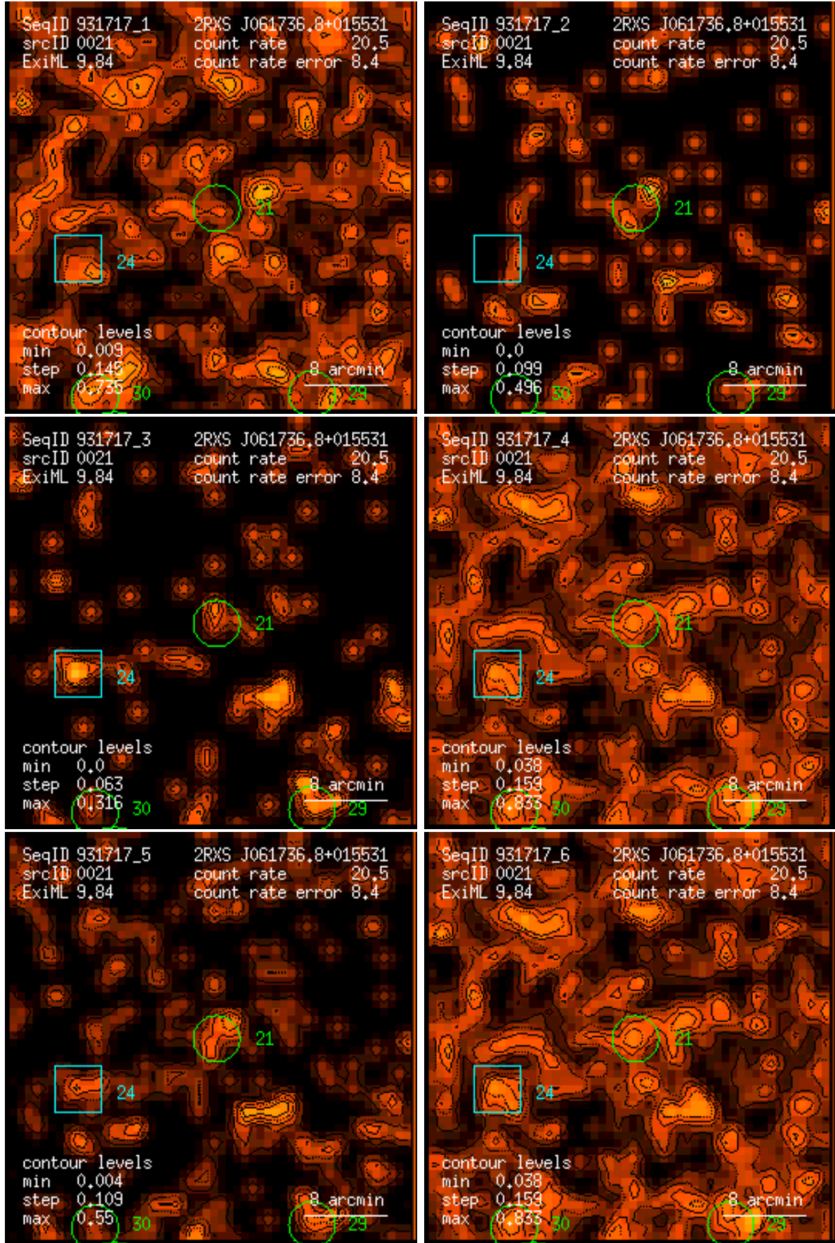
Figure 21: RASS 931717: detection 0021: band rate images, Gaussian filter: (1) PSPC channels 11 – 41, (2) 52 – 90, (3) 91 – 201, (4) 11 – 235, (5) 52 – 201, (6) 11 – 201. Broad band rates in counts/ks. Band rate contour levels in counts/ks/arcmin 2 .
