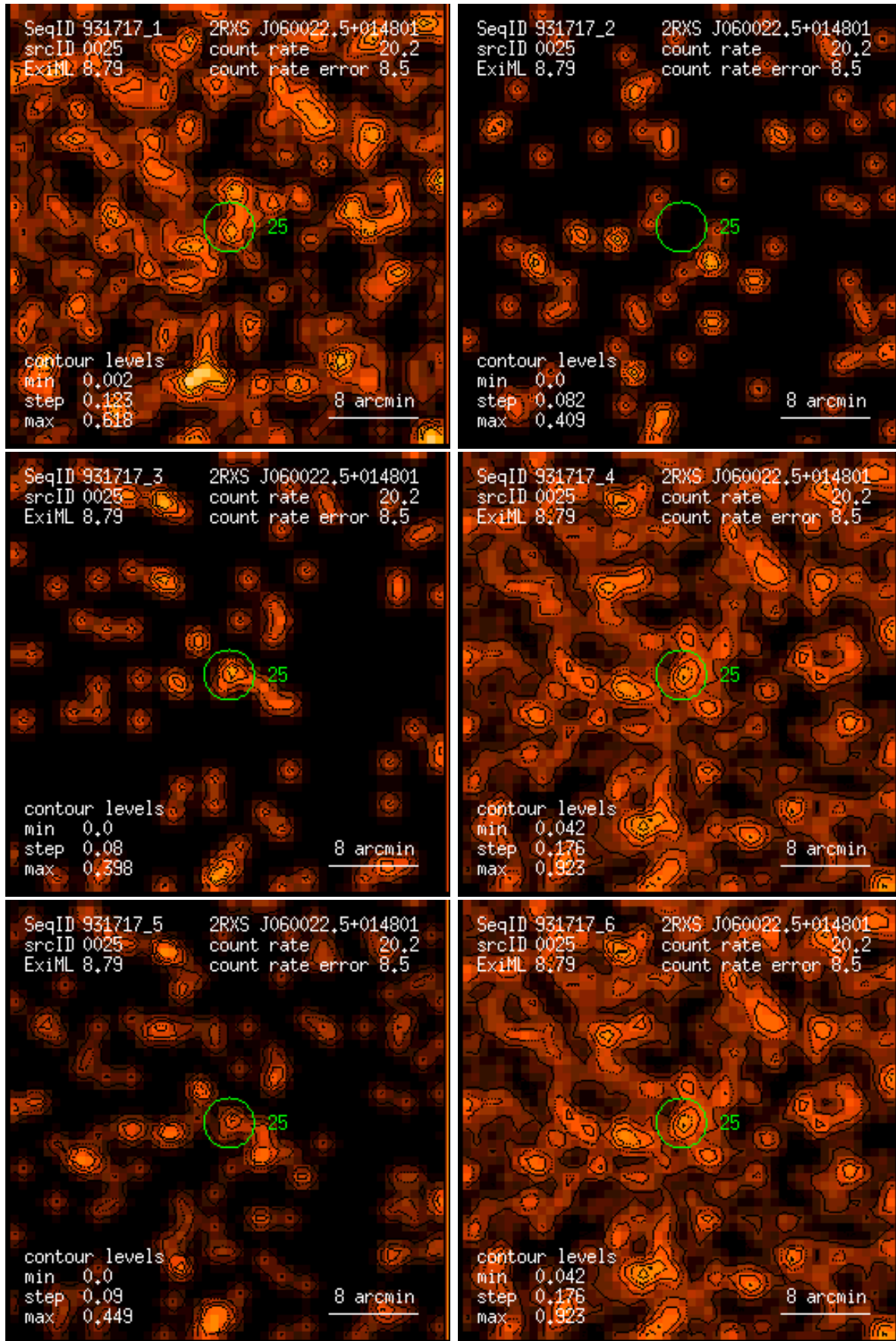
Figure 25: RASS 931717: detection 0025: band rate images, Gaussian filter: (1) PSPC channels 11 – 41, (2) 52 – 90, (3) 91 – 201, (4) 11 – 235, (5) 52 – 201, (6) 11 – 201. Broad band rates in counts/ks. Band rate contour levels in counts/ks/arcmin 2 .
