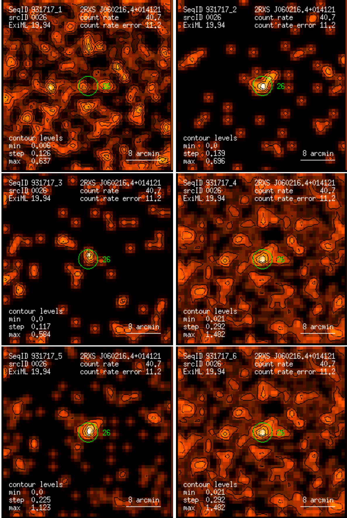
Figure 26: RASS 931717: detection 0026: band rate images, Gaussian filter: (1) PSPC channels 11 – 41, (2) 52 – 90, (3) 91 – 201, (4) 11 – 235, (5) 52 – 201, (6) 11 – 201. Broad band rates in counts/ks. Band rate contour levels in counts/ks/arcmin 2 .
