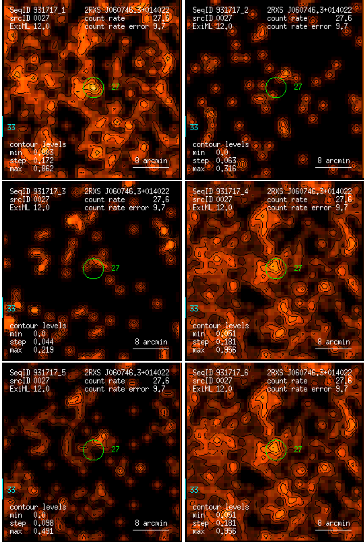
Figure 27: RASS 931717: detection 0027: band rate images, Gaussian filter: (1) PSPC channels 11 – 41, (2) 52 – 90, (3) 91 – 201, (4) 11 – 235, (5) 52 – 201, (6) 11 – 201. Broad band rates in counts/ks. Band rate contour levels in counts/ks/arcmin 2 .
