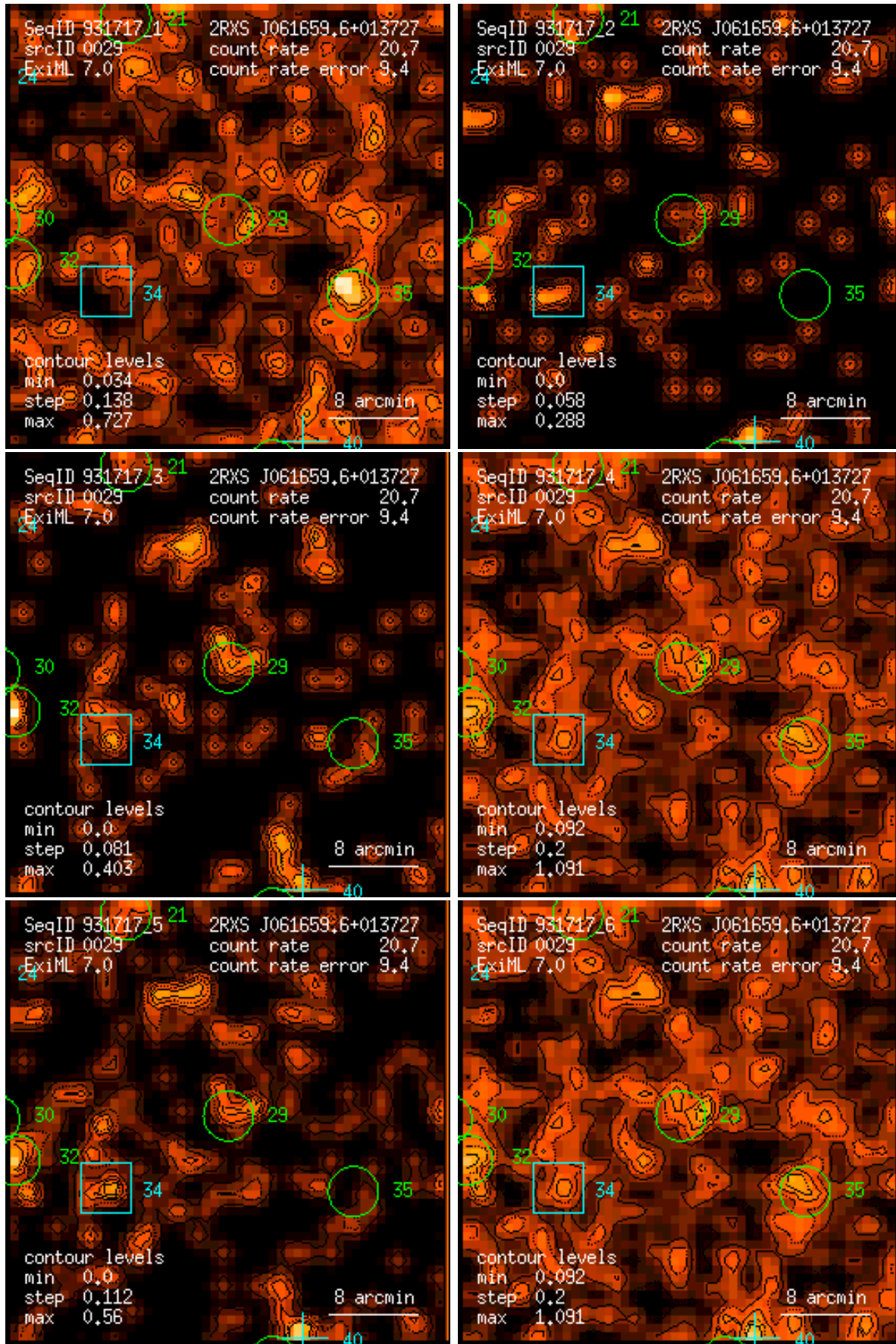
Figure 29: RASS 931717: detection 0029: band rate images, Gaussian filter: (1) PSPC channels 11 – 41, (2) 52 – 90, (3) 91 – 201, (4) 11 – 235, (5) 52 – 201, (6) 11 – 201. Broad band rates in counts/ks. Band rate contour levels in counts/ks/arcmin 2 .
