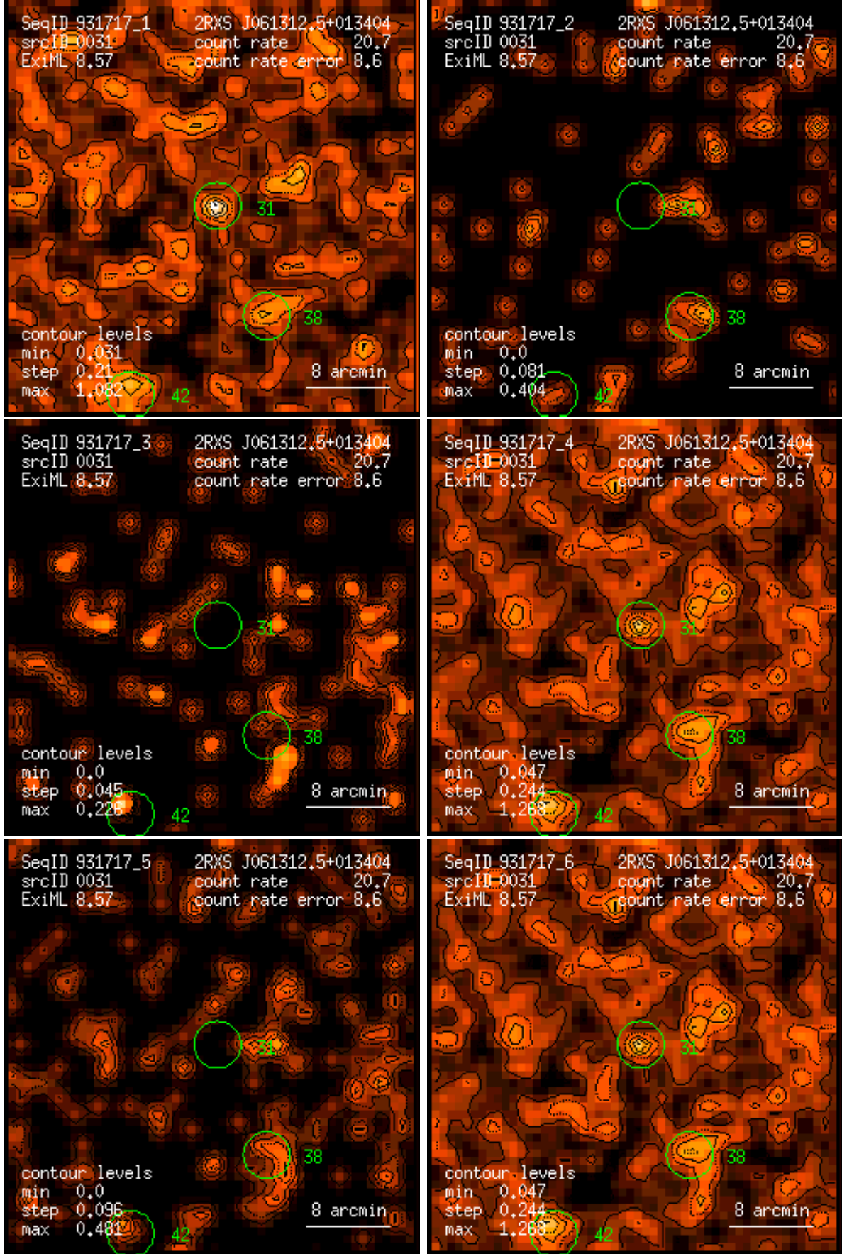
Figure 31: RASS 931717: detection 0031: band rate images, Gaussian filter: (1) PSPC channels 11 – 41, (2) 52 – 90, (3) 91 – 201, (4) 11 – 235, (5) 52 – 201, (6) 11 – 201. Broad band rates in counts/ks. Band rate contour levels in counts/ks/arcmin 2 .
