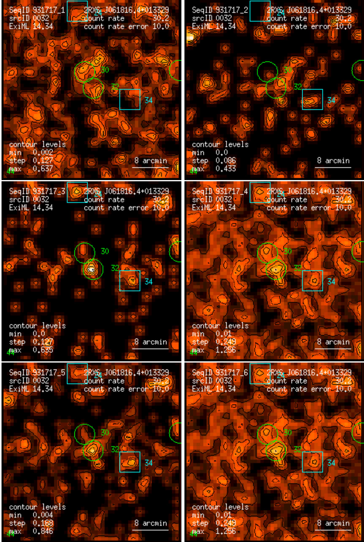
Figure 32: RASS 931717: detection 0032: band rate images, Gaussian filter: (1) PSPC channels 11 – 41, (2) 52 – 90, (3) 91 – 201, (4) 11 – 235, (5) 52 – 201, (6) 11 – 201. Broad band rates in counts/ks. Band rate contour levels in counts/ks/arcmin 2 .
