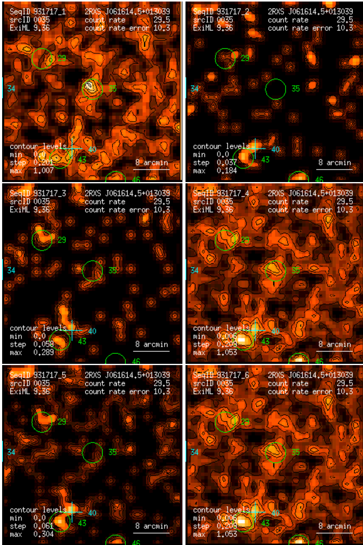
Figure 35: RASS 931717: detection 0035: band rate images, Gaussian filter: (1) PSPC channels 11 – 41, (2) 52 – 90, (3) 91 – 201, (4) 11 – 235, (5) 52 – 201, (6) 11 – 201. Broad band rates in counts/ks. Band rate contour levels in counts/ks/arcmin 2 .
