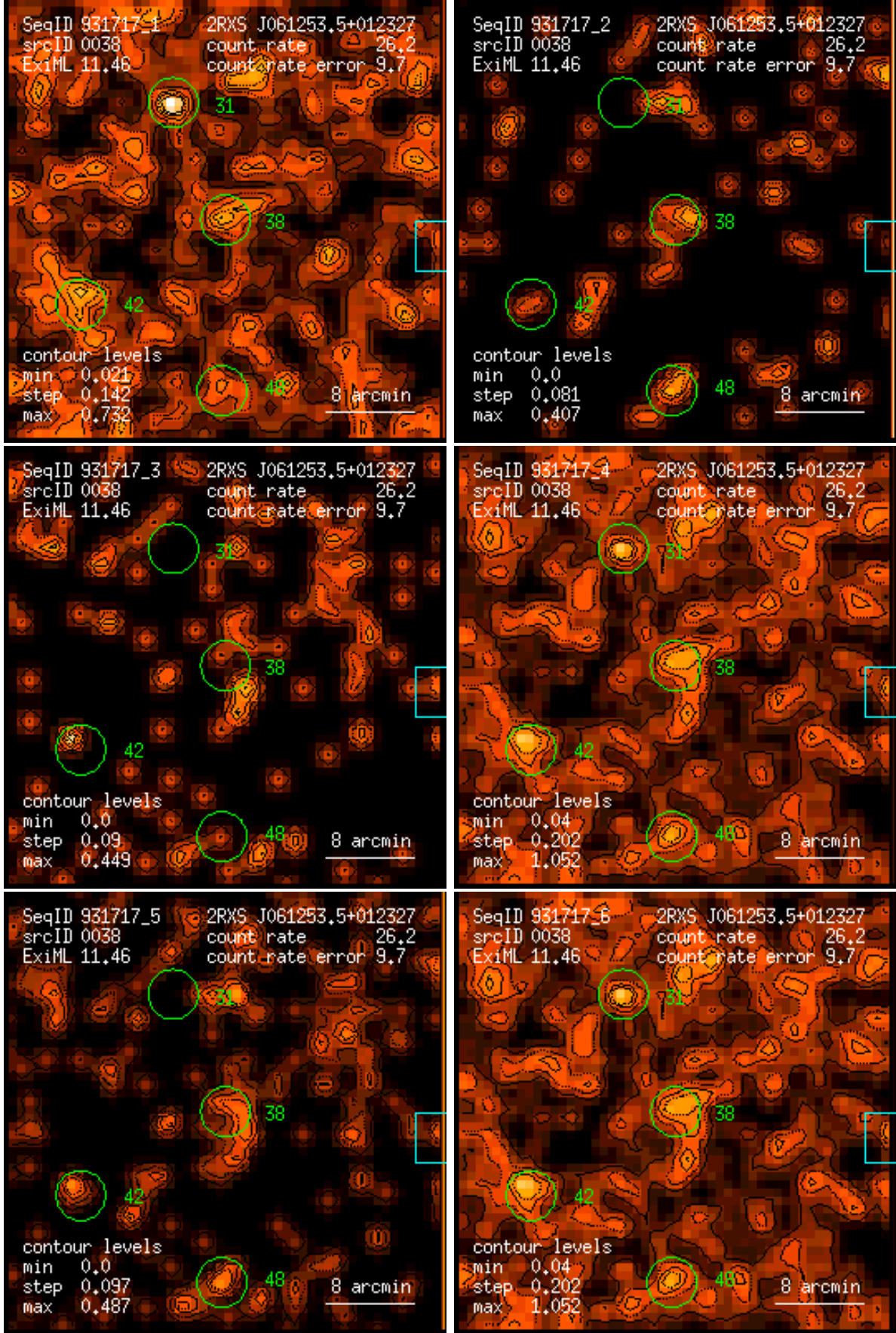
Figure 38: RASS 931717: detection 0038: band rate images, Gaussian filter: (1) PSPC channels 11 – 41, (2) 52 – 90, (3) 91 – 201, (4) 11 – 235, (5) 52 – 201, (6) 11 – 201. Broad band rates in counts/ks. Band rate contour levels in counts/ks/arcmin 2 .
