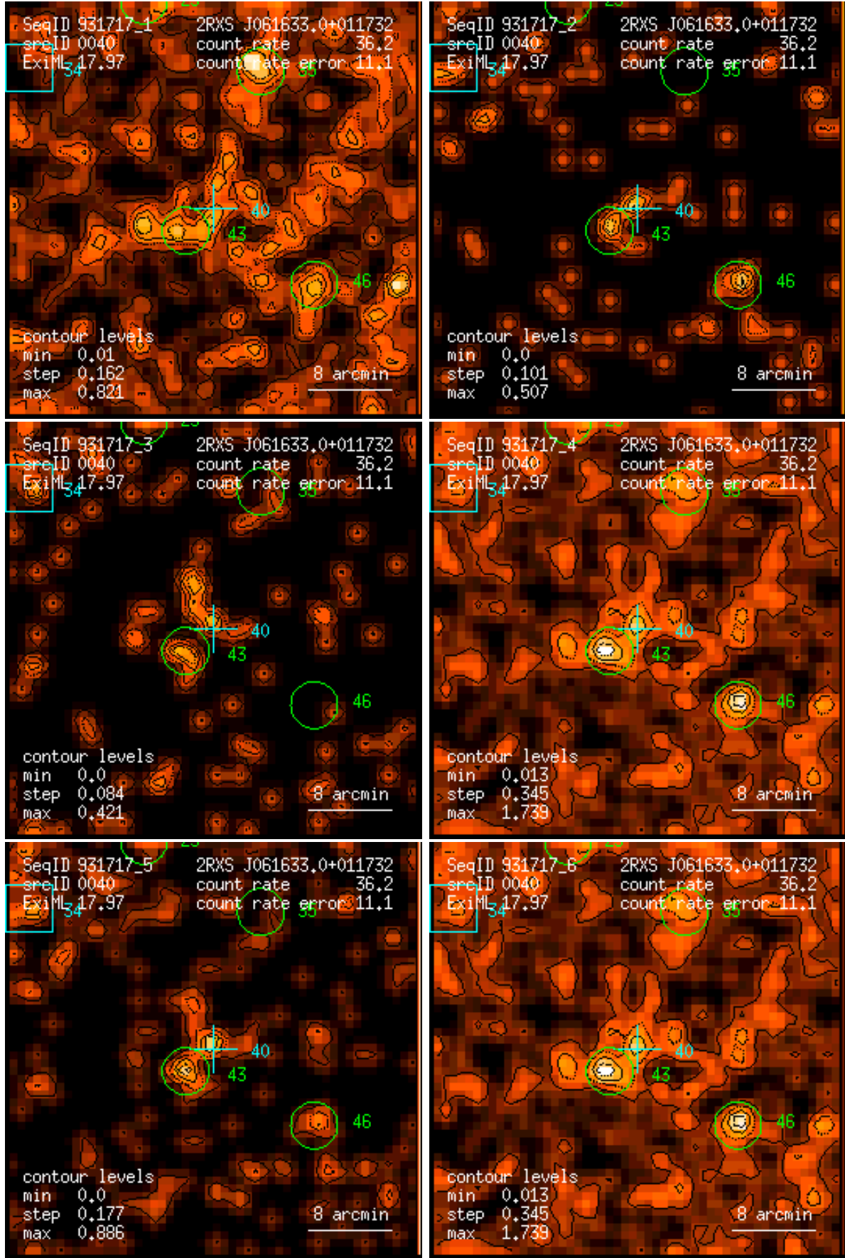
Figure 40: RASS 931717: detection 0040: band rate images, Gaussian filter: (1) PSPC channels 11 – 41, (2) 52 – 90, (3) 91 – 201, (4) 11 – 235, (5) 52 – 201, (6) 11 – 201. Broad band rates in counts/ks. Band rate contour levels in counts/ks/arcmin 2 .
