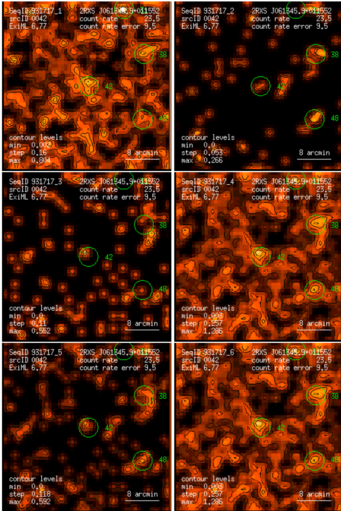
Figure 42: RASS 931717: detection 0042: band rate images, Gaussian filter: (1) PSPC channels 11 – 41, (2) 52 – 90, (3) 91 – 201, (4) 11 – 235, (5) 52 – 201, (6) 11 – 201. Broad band rates in counts/ks. Band rate contour levels in counts/ks/arcmin 2 .
