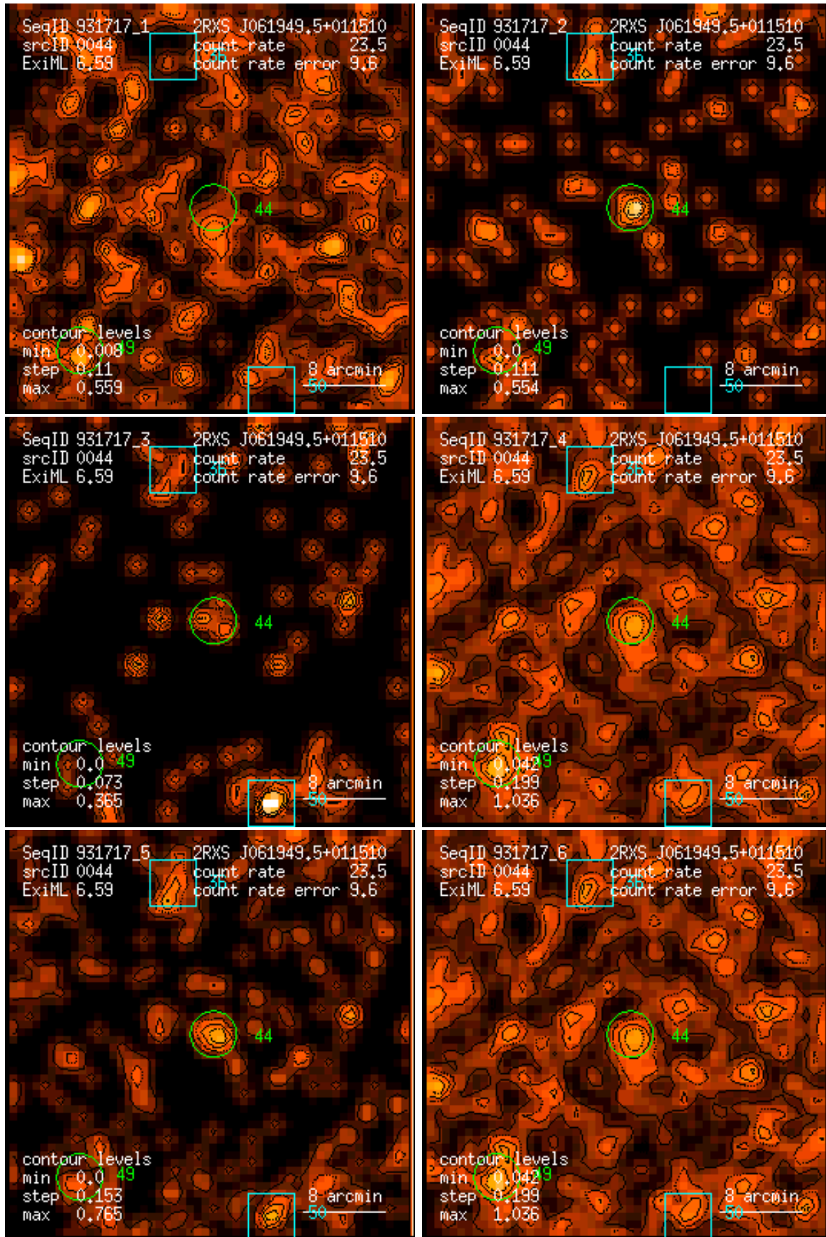
Figure 44: RASS 931717: detection 0044: band rate images, Gaussian filter: (1) PSPC channels 11 – 41, (2) 52 – 90, (3) 91 – 201, (4) 11 – 235, (5) 52 – 201, (6) 11 – 201. Broad band rates in counts/ks. Band rate contour levels in counts/ks/arcmin 2 .
