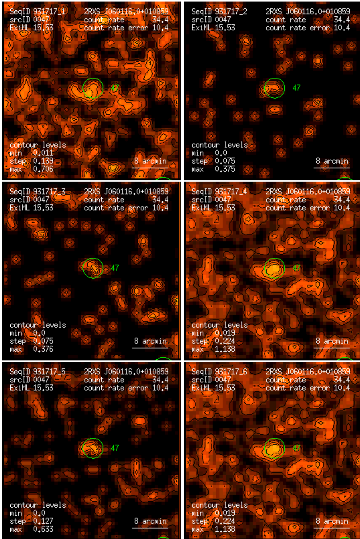
Figure 47: RASS 931717: detection 0047: band rate images, Gaussian filter: (1) PSPC channels 11 – 41, (2) 52 – 90, (3) 91 – 201, (4) 11 – 235, (5) 52 – 201, (6) 11 – 201. Broad band rates in counts/ks. Band rate contour levels in counts/ks/arcmin 2 .
