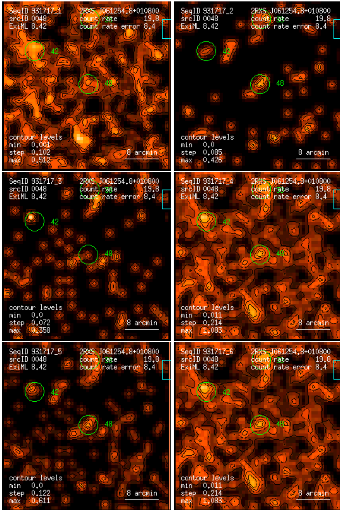
Figure 48: RASS 931717: detection 0048: band rate images, Gaussian filter: (1) PSPC channels 11 – 41, (2) 52 – 90, (3) 91 – 201, (4) 11 – 235, (5) 52 – 201, (6) 11 – 201. Broad band rates in counts/ks. Band rate contour levels in counts/ks/arcmin 2 .
