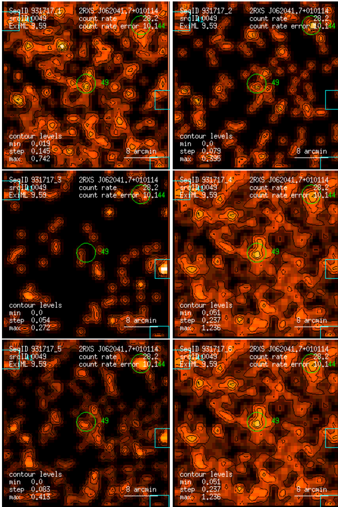
Figure 49: RASS 931717: detection 0049: band rate images, Gaussian filter: (1) PSPC channels 11 – 41, (2) 52 – 90, (3) 91 – 201, (4) 11 – 235, (5) 52 – 201, (6) 11 – 201. Broad band rates in counts/ks. Band rate contour levels in counts/ks/arcmin 2 .
