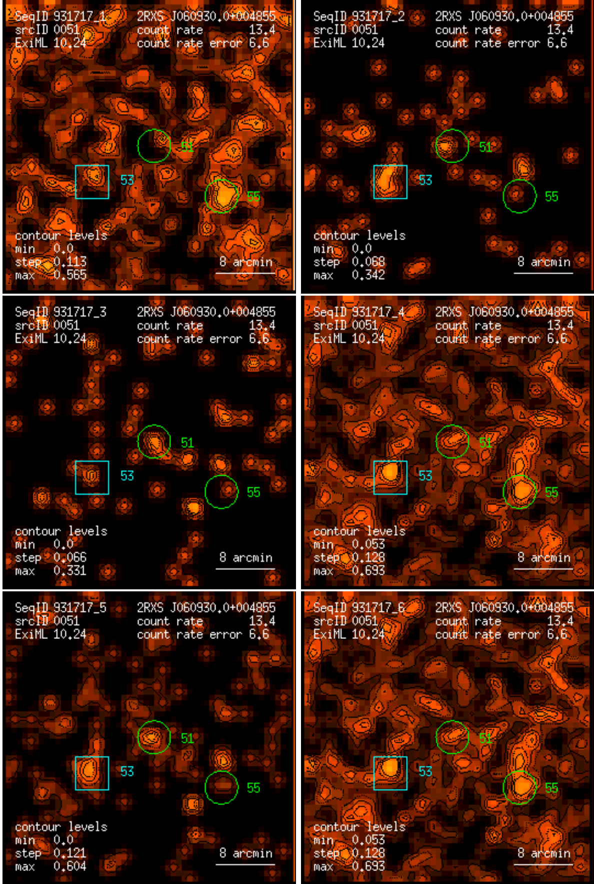
Figure 51: RASS 931717: detection 0051: band rate images, Gaussian filter: (1) PSPC channels 11 – 41, (2) 52 – 90, (3) 91 – 201, (4) 11 – 235, (5) 52 – 201, (6) 11 – 201. Broad band rates in counts/ks. Band rate contour levels in counts/ks/arcmin 2 .
