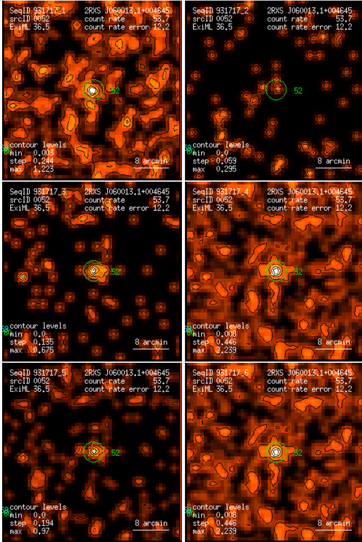
Figure 52: RASS 931717: detection 0052: band rate images, Gaussian filter: (1) PSPC channels 11 – 41, (2) 52 – 90, (3) 91 – 201, (4) 11 – 235, (5) 52 – 201, (6) 11 – 201. Broad band rates in counts/ks. Band rate contour levels in counts/ks/arcmin 2 .
